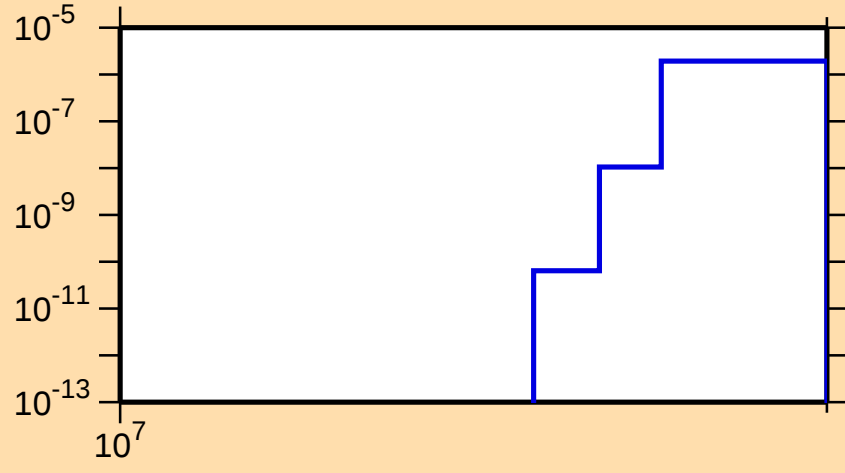
\sigma vs. E for ^{90}\text{Tc}(n,\text{pt})
