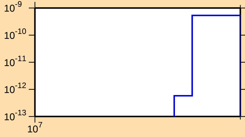
\sigma vs. E for ^{90}\text{Tc}(\text{mt } 34)
