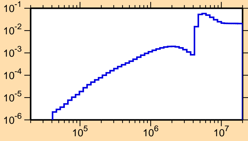
\sigma vs. E for ^{90}\text{Tc}(n,n\text{cont.})
