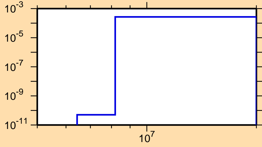
\sigma vs. E for ^{90}\text{Tc}(n,\text{He}3)
