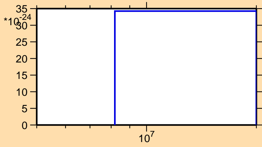
\sigma vs. E for ^{90}\text{Tc}(n,nt)
