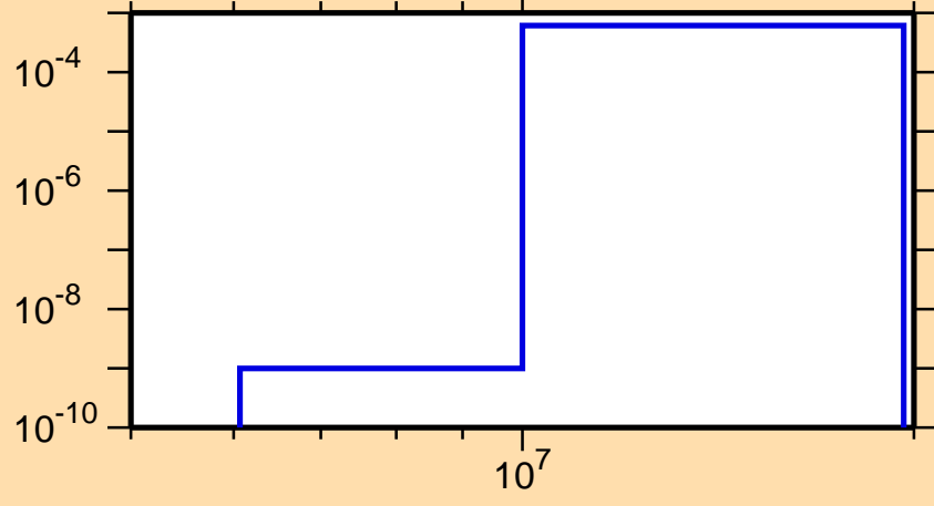
\sigma vs. E for ^{90}\text{Tc}(n,t)
