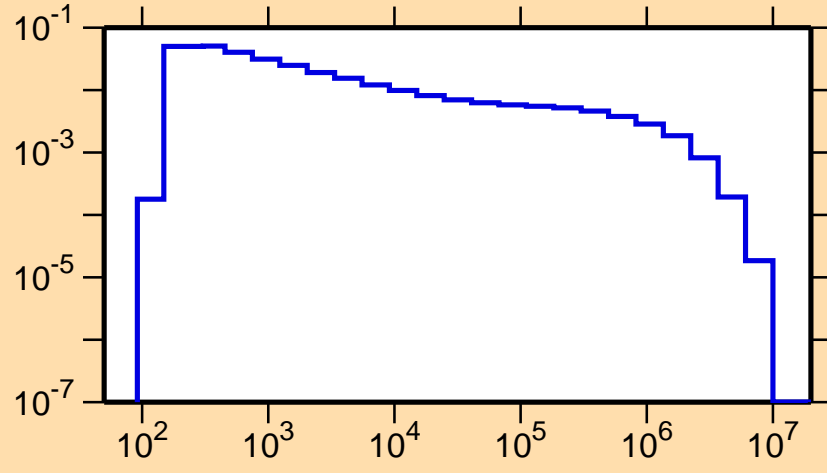
\sigma vs. E for ^{90}\text{Tc}(n,n_3)
