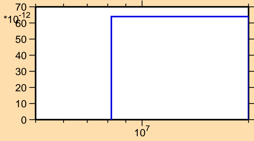
\sigma vs. E for ^{90}\text{Tc} (mt 34)
