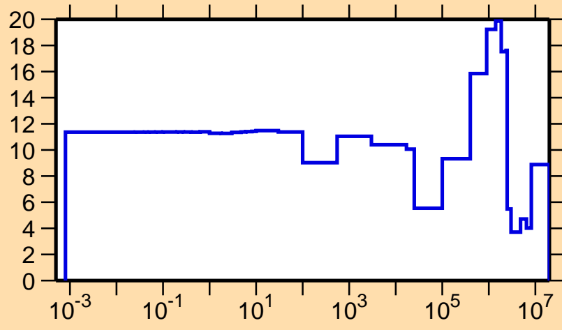
\Delta\sigma/\sigma vs. E for ^{90}\text{Tc}(n,el.)
