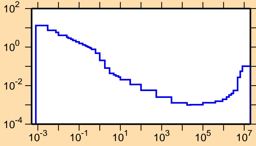
\sigma vs. E for ^{90}\text{Tc}(n,\alpha)
