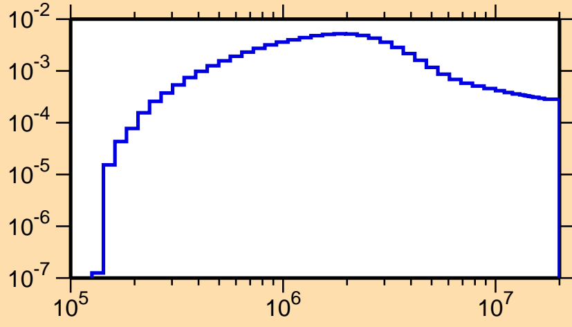
\sigma vs. E for ^{91}\text{Tc}(n,n_1)
