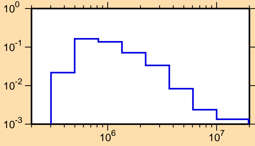
\sigma vs. E for ^{91}\text{Tc}(n,n_2)
