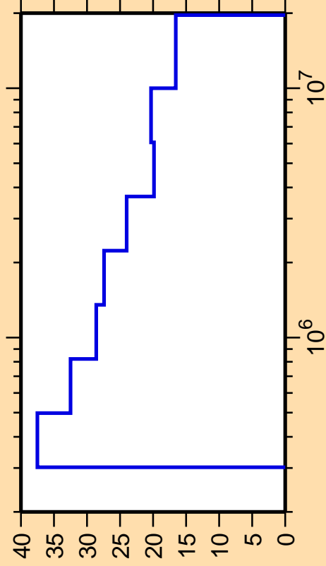
\Delta\sigma/\sigma vs. E for ^{91}\text{Tc}(n,n_2)
