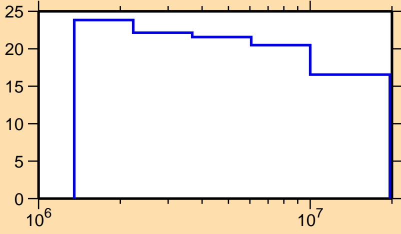
\Delta\sigma/\sigma vs. E for ^{91}\text{Tc}(n,n_1)
