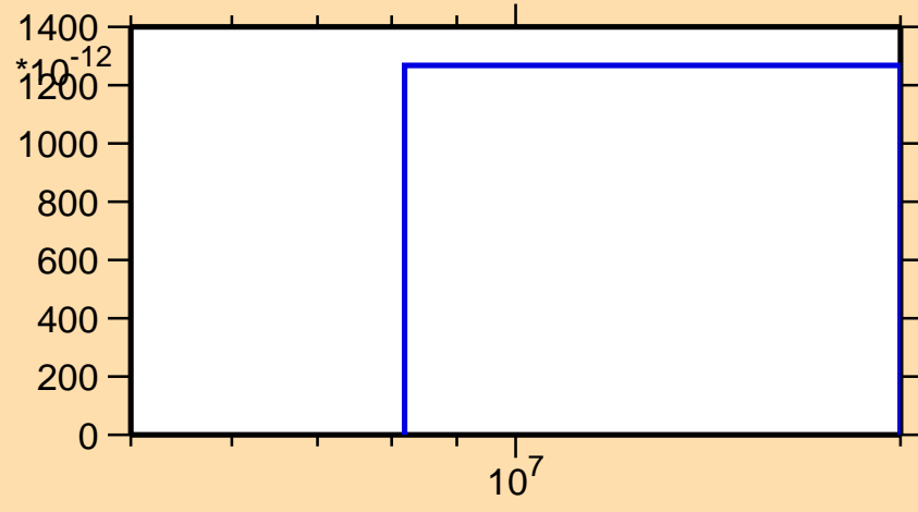
\sigma vs. E for ^{91}\text{Tc}(\text{mt } 45)
