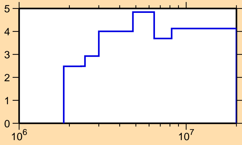
\Delta\sigma/\sigma vs. E for ^{91}\text{Tc}(n,n\text{onel.})
