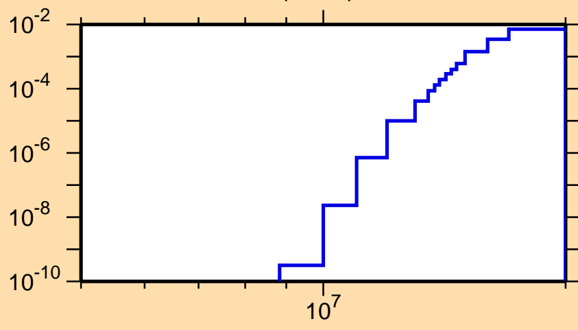
\sigma vs. E for ^{91}\text{Tc}(n,n\alpha)
