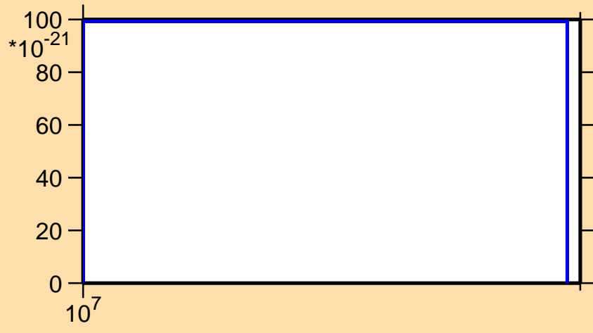
\sigma vs. E for ^{92}\text{Tc}(n,nt)
