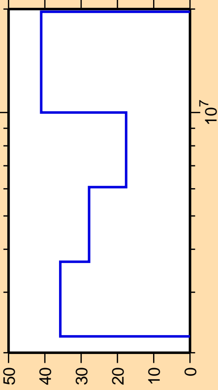
\Delta\sigma/\sigma vs. E for ^{92}\text{Tc}(n,n\text{cont.})
