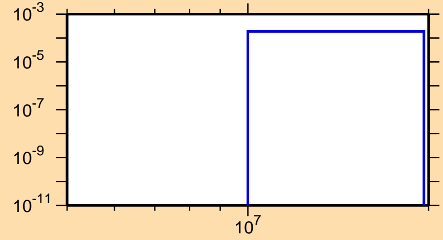
\sigma vs. E for ^{92}\text{Tc}(n,\alpha)
