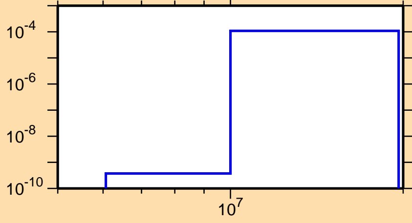
\sigma vs. E for ^{92}\text{Tc}(n,t)
