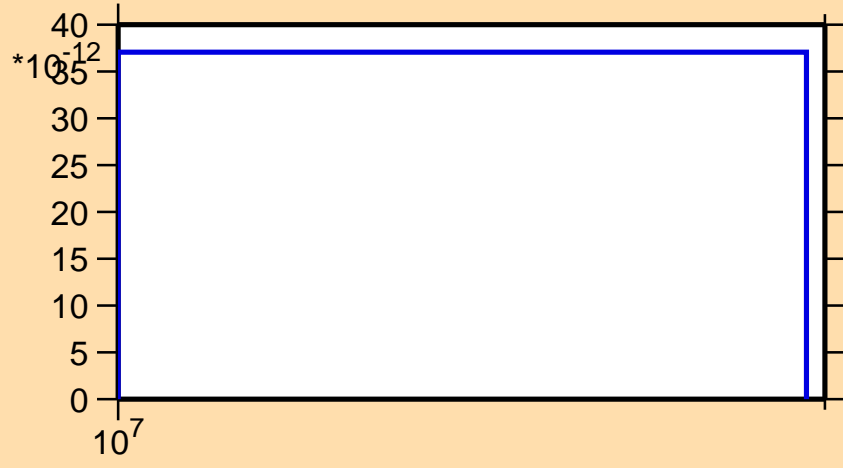
\sigma vs. E for ^{92}\text{Tc} (mt 45)
