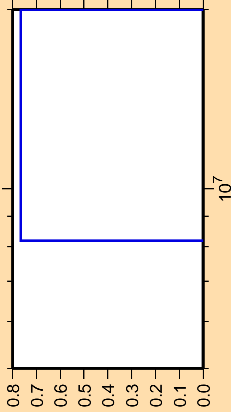
\Delta\sigma/\sigma vs. E for ^{92}\text{Tc}(\text{mt } 34)
