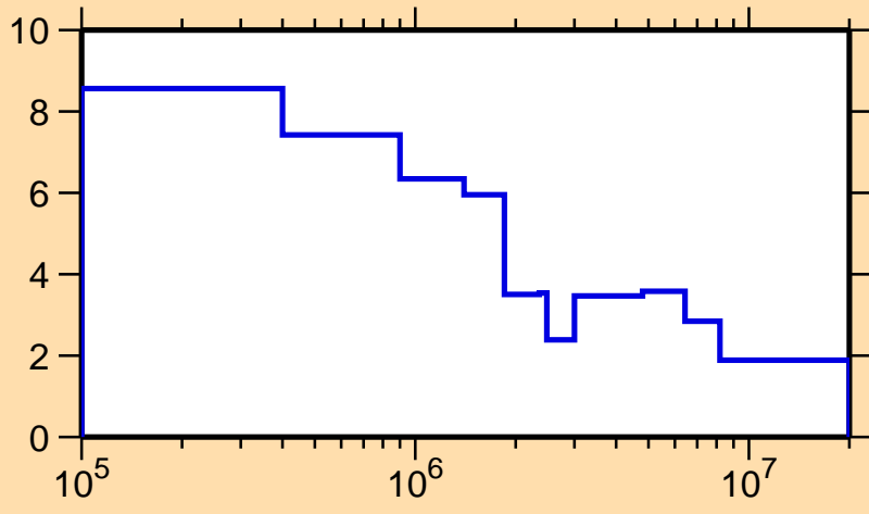
\Delta\sigma/\sigma vs. E for ^{92}\text{Tc}(n,\text{tot.})
