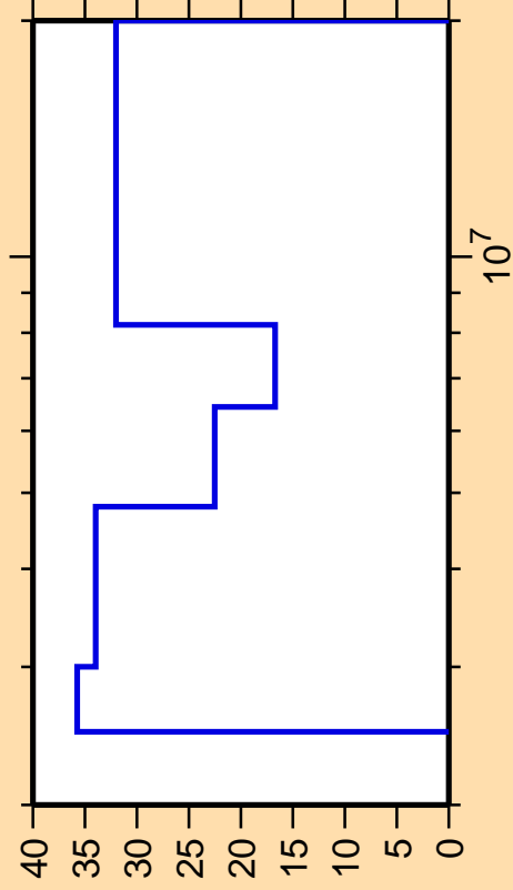
\Delta\sigma/\sigma vs. E for ^{92}\text{Tc}(n,\text{ncont.})
