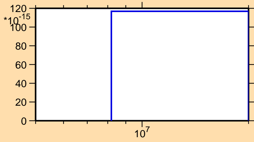
\sigma vs. E for ^{92}\text{Tc}(\text{mt } 34)
