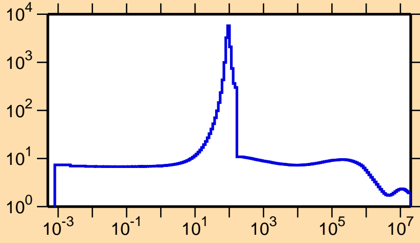
\sigma vs. E for ^{93}\text{Tc}(n,\text{el.})
