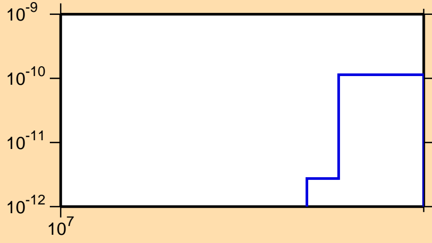
\sigma vs. E for ^{93}\text{Tc}(\text{mt117})
