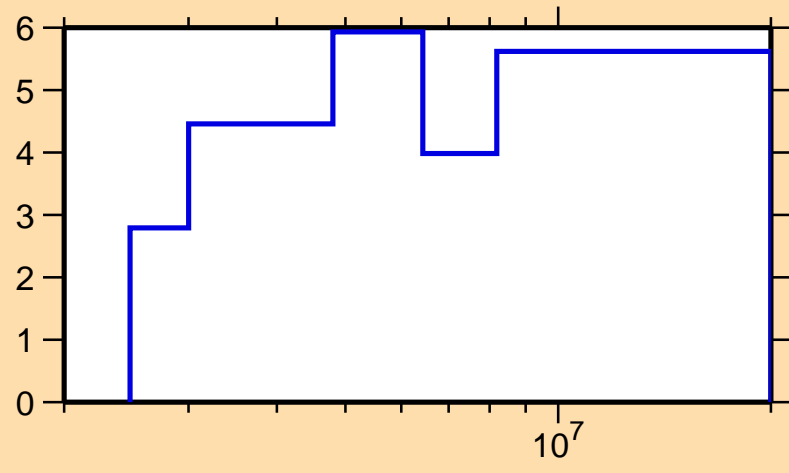
\Delta\sigma/\sigma vs. E for ^{93}\text{Tc}(n, el.)
