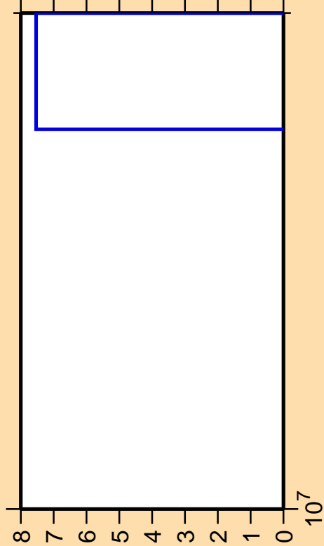
\Delta\sigma/\sigma vs. E for ^{94}\text{Tc}(n,nt)
