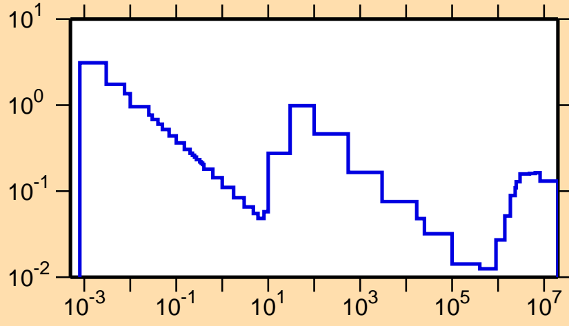
\sigma vs. E for ^{94}\text{Tc}(n,p)
