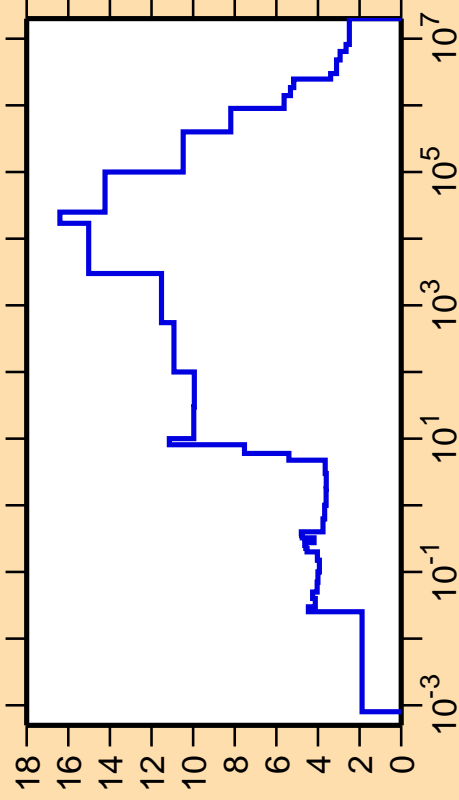
\Delta\sigma/\sigma vs. E for ^{94}\text{Tc}(n,\text{nonel.})
