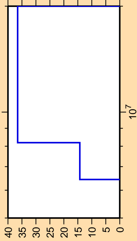
\Delta\sigma/\sigma vs. E for ^{94}\text{Tc}(n,n\alpha)
