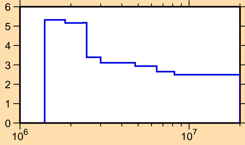
\Delta\sigma/\sigma vs. E for ^{94}\text{Tc}(n,\text{nonel.})
