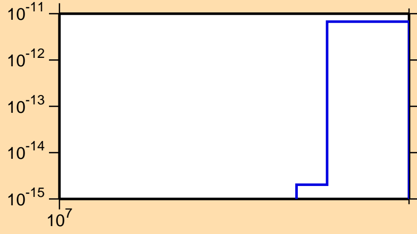
\sigma vs. E for ^{94}\text{Tc}(n,2n\alpha)
