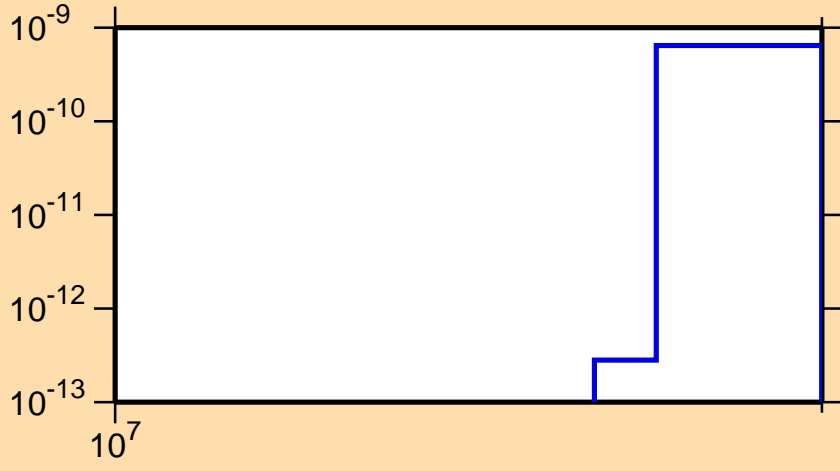
\sigma vs. E for ^{94}\text{Tc} (mt 34)
