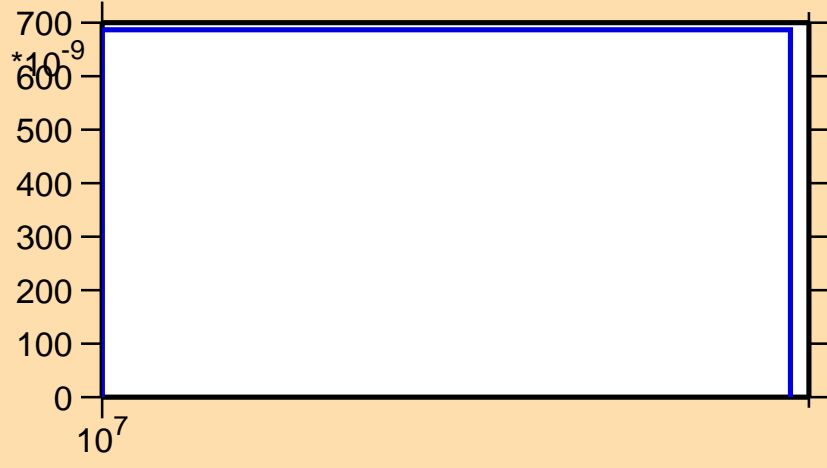
\sigma vs. E for ^{95}\text{Tc}(n,nd)
