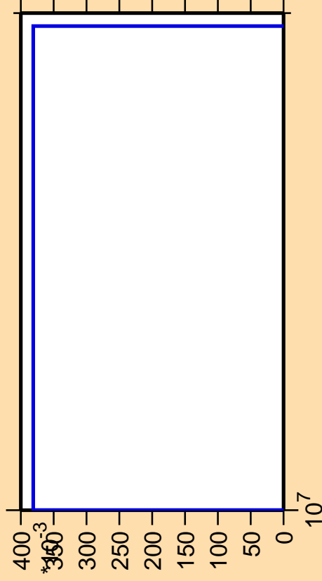
\Delta\sigma/\sigma vs. E for ^{95}\text{Tc}(n,\text{pt})
