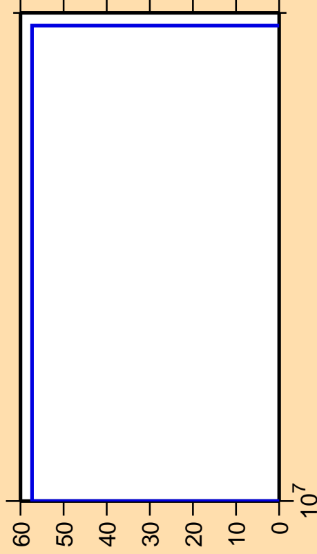
\Delta\sigma/\sigma vs. E for ^{95}\text{Tc}(n,nd)
