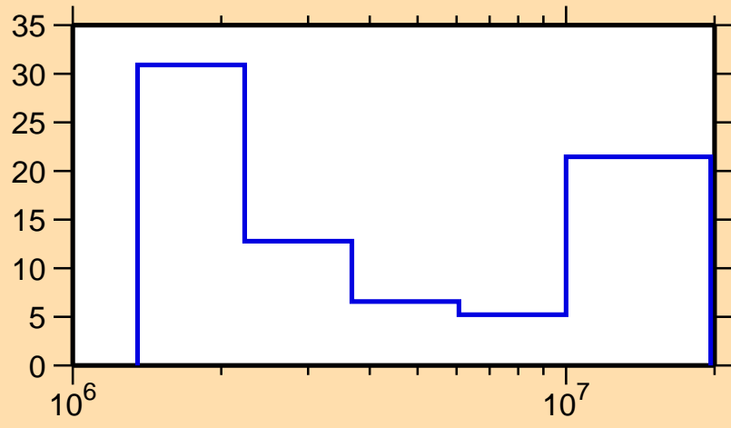
\Delta\sigma/\sigma vs. E for ^{95}\text{Tc}(n,ncont.)
