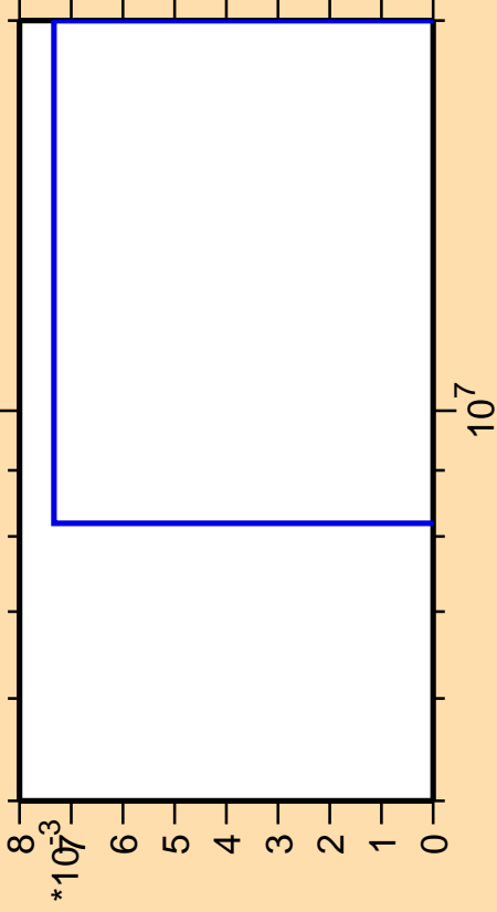
\Delta\sigma/\sigma vs. E for ^{95}\text{Tc}(\text{mt } 34)
