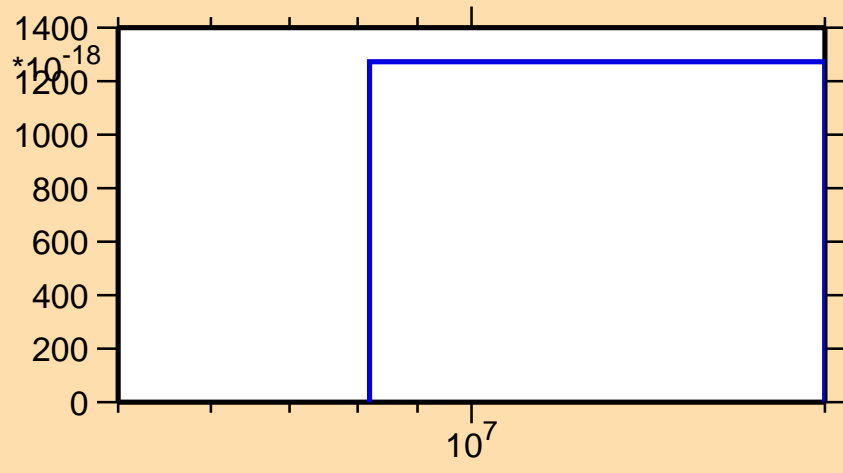
\sigma vs. E for ^{95}\text{Tc}(\text{mt } 34)
