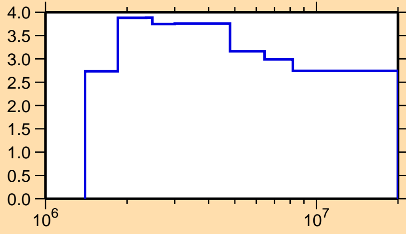
\Delta\sigma/\sigma vs. E for ^{95}\text{Tc}(n,n\text{nonel.})
