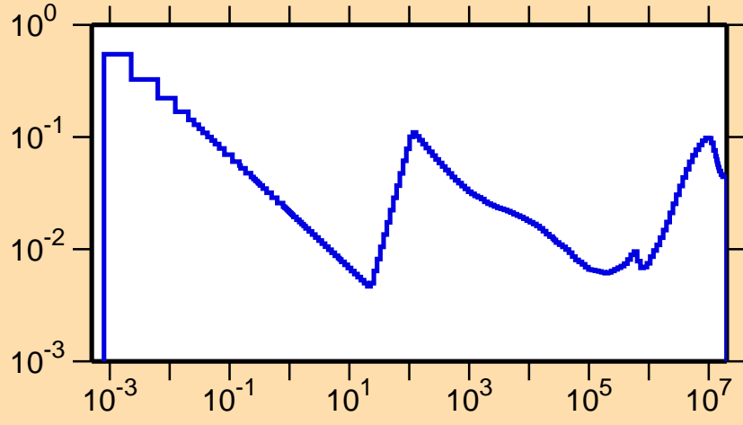
\sigma vs. E for ^{95}\text{Tc}(n,p)
