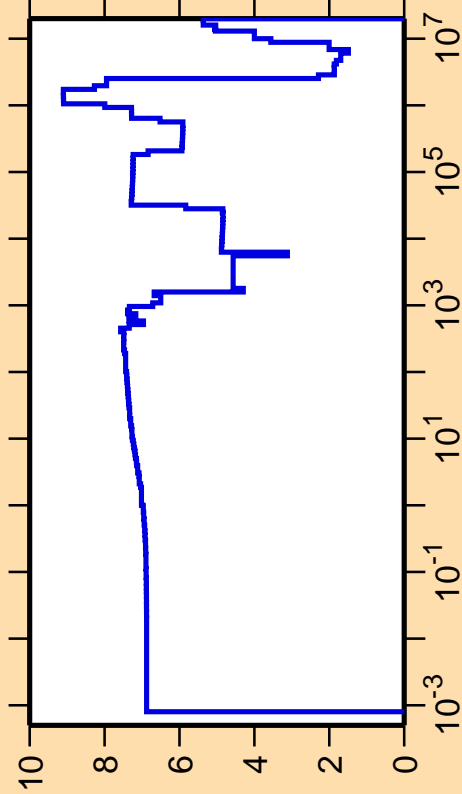
\Delta\sigma/\sigma vs. E for ^{95}\text{Tc}(n,\text{el.})
