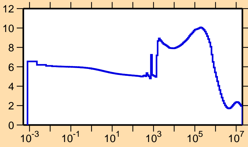
\sigma vs. E for ^{95}\text{Tc}(n,\text{el.})
