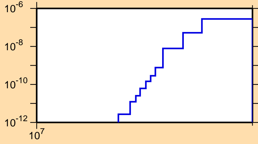
\sigma vs. E for ^{95}\text{Tc}(\text{mt117})
