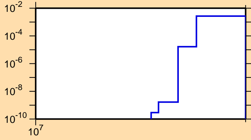
\sigma vs. E for ^{95}\text{Tc}(n,2np)
