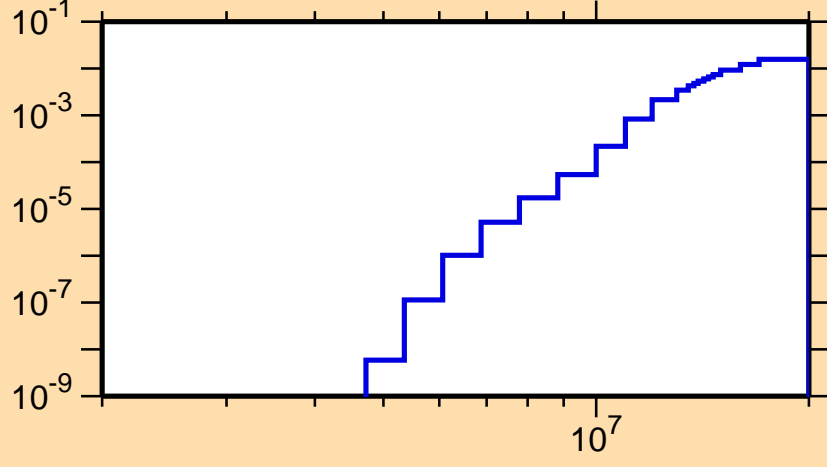
\sigma vs. E for ^{95}\text{Tc}(n,d)
