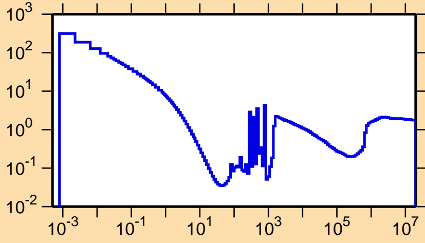
\sigma vs. E for ^{95}\text{Tc}(n,\text{nonel.})
