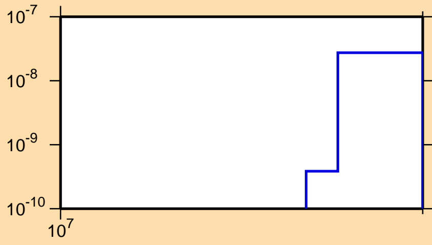
\sigma vs. E for ^{95}\text{Tc}(n,\text{pd})
