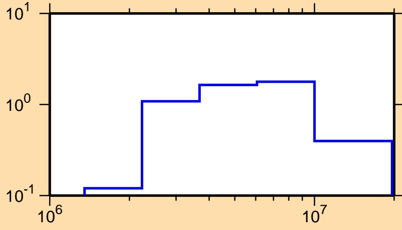
\sigma vs. E for ^{95}\text{Tc}(n,n\text{cont.})
