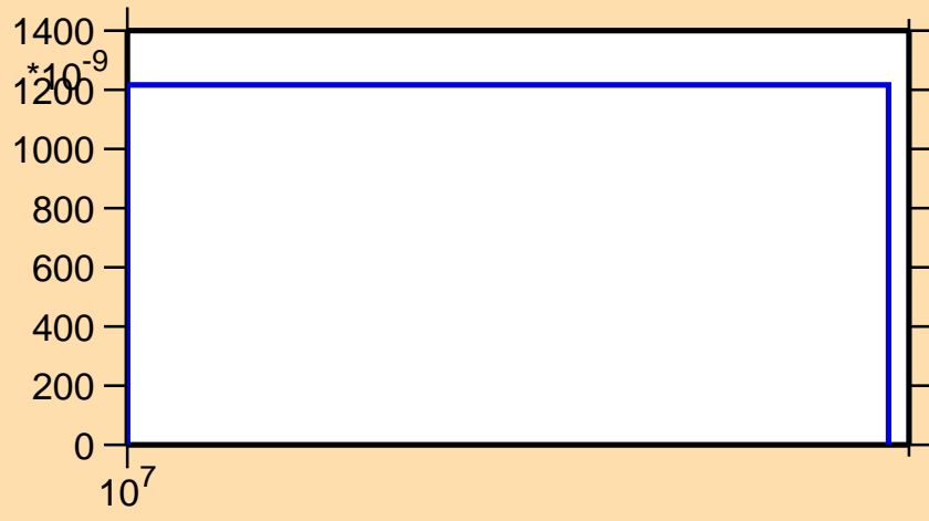
\sigma vs. E for ^{95}\text{Tc}(n,\text{nd})
