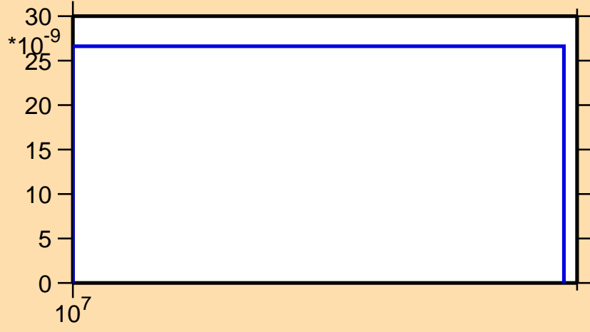
\sigma vs. E for ^{95}\text{Tc} (mt 45)
