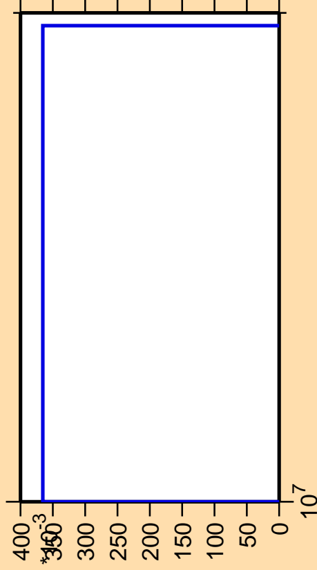
\Delta\sigma/\sigma vs. E for ^{95}\text{Tc}(n,2n\alpha)
