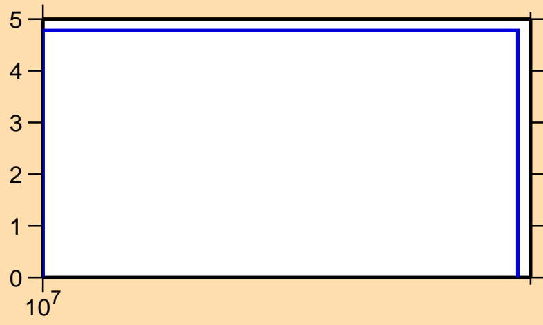
\Delta\sigma/\sigma vs. E for ^{95}\text{Tc}(n,\text{el.})
