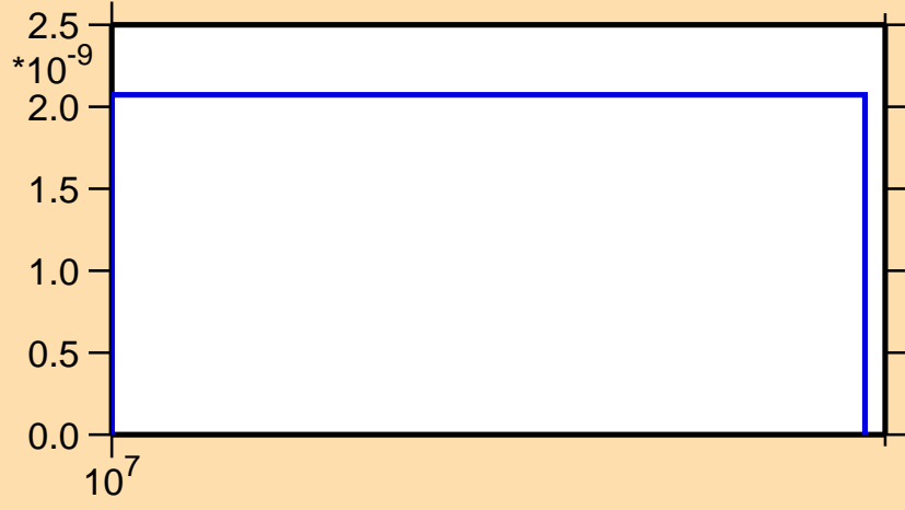
\sigma vs. E for ^{95}\text{Tc}(n,nt)
