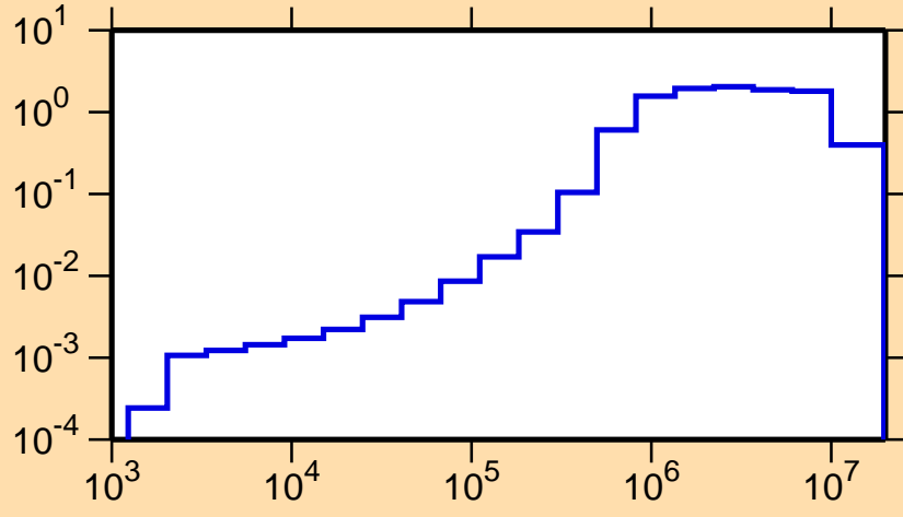
\sigma vs. E for ^{95}\text{Tc}(n,\text{inel.})
