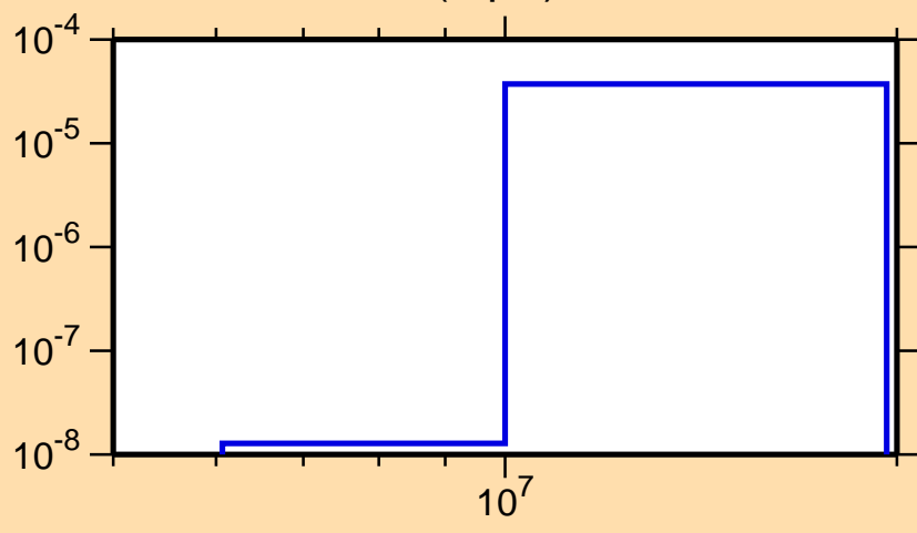
\sigma vs. E for ^{95}\text{Tc}(n,p\alpha)
