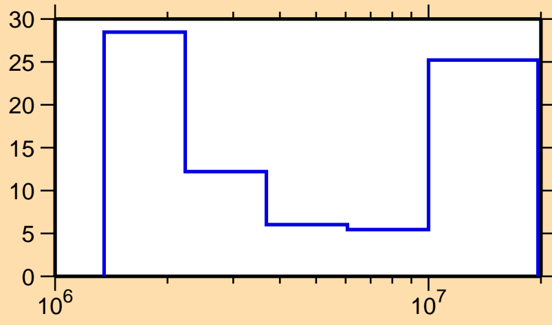
\Delta\sigma/\sigma vs. E for ^{95}\text{Tc}(n,n\text{cont.})
