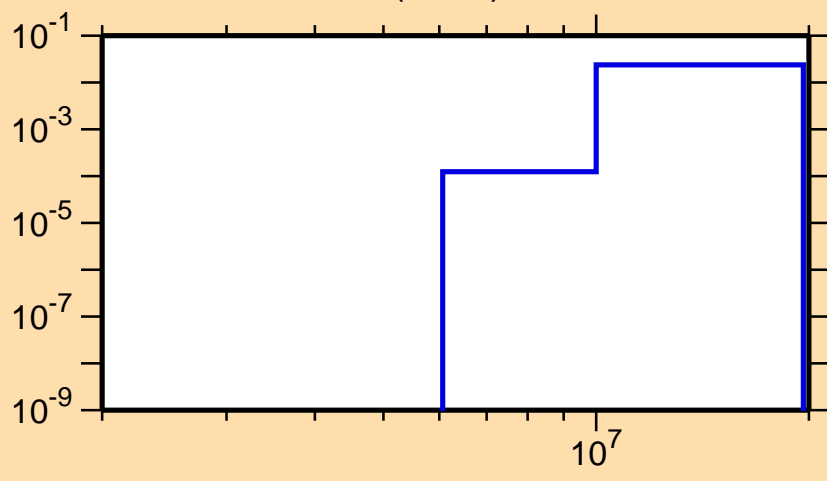
\sigma vs. E for ^{95}\text{Tc}(n,n\alpha)
