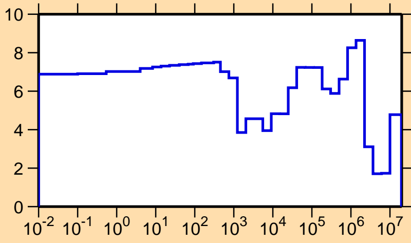
\Delta\sigma/\sigma vs. E for ^{95}\text{Tc}(n,el.)
