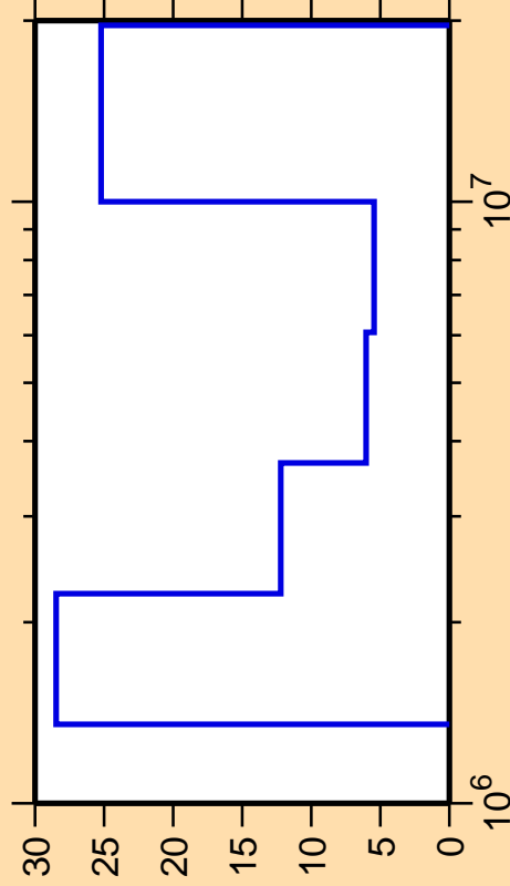
\Delta\sigma/\sigma vs. E for ^{95}\text{Tc}(n,n\text{cont.})
