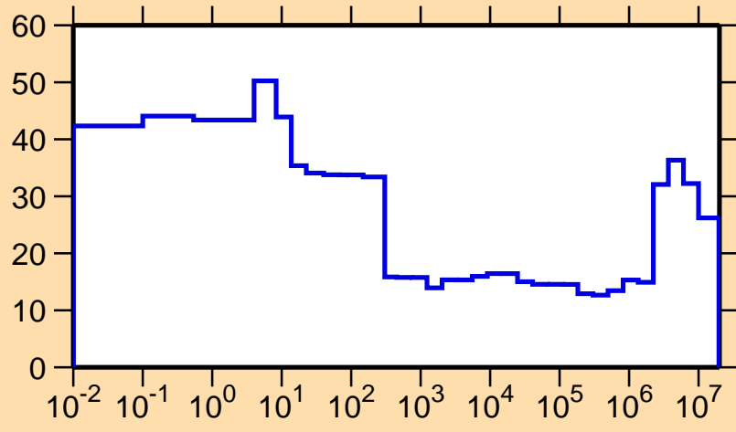
\Delta\sigma/\sigma vs. E for ^{95}\text{Tc}(n,p)
