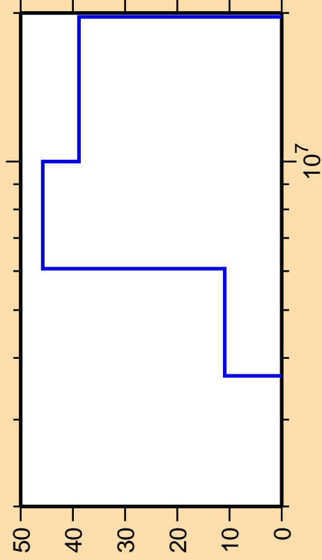
\Delta\sigma/\sigma vs. E for ^{95}\text{Tc}(n,n\alpha)
