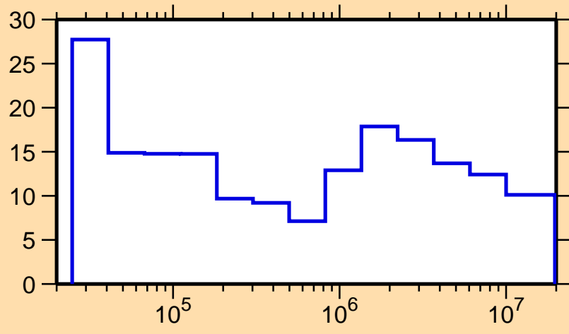
\Delta\sigma/\sigma vs. E for ^{96}\text{Tc}(n,n_1)
