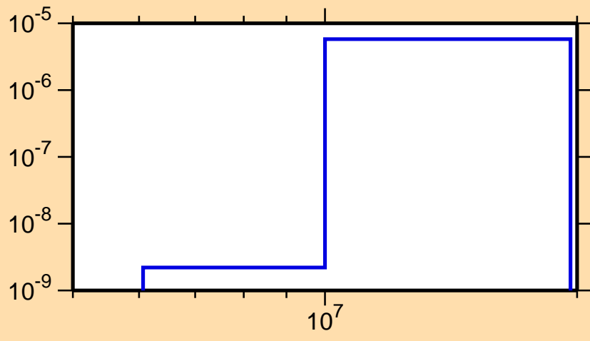
\sigma vs. E for ^{96}\text{Tc}(n,p\alpha)
