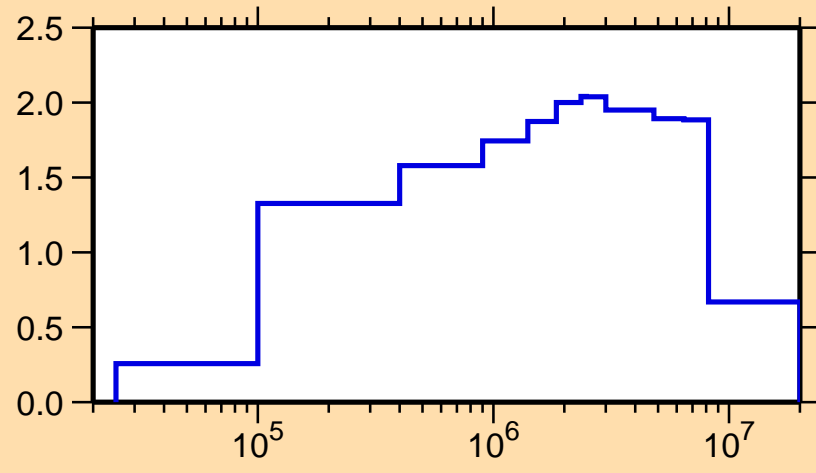
\sigma vs. E for ^{96}\text{Tc}(n,\text{inel.})
