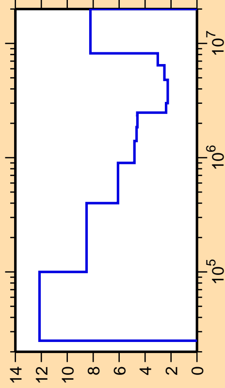
\Delta\sigma/\sigma vs. E for ^{96}\text{Tc}(n,\text{inel.})
