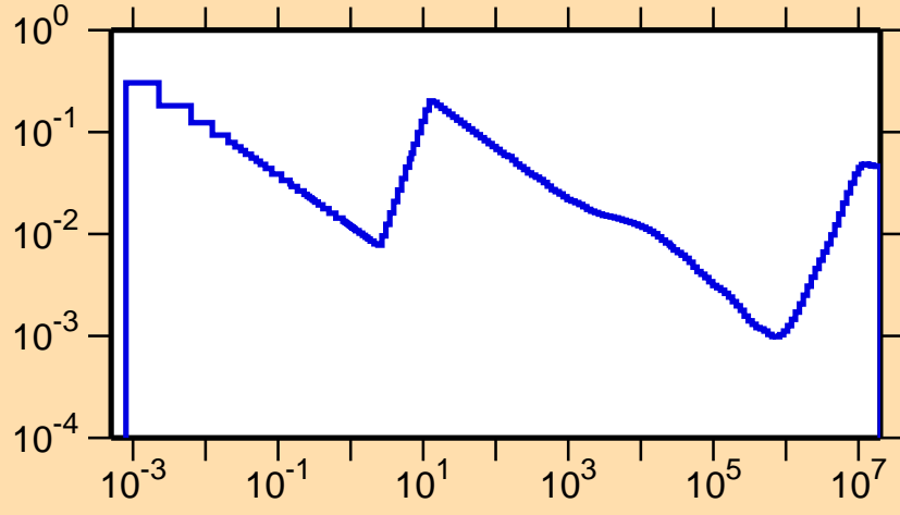
\sigma vs. E for ^{96}\text{Tc}(n,p)
