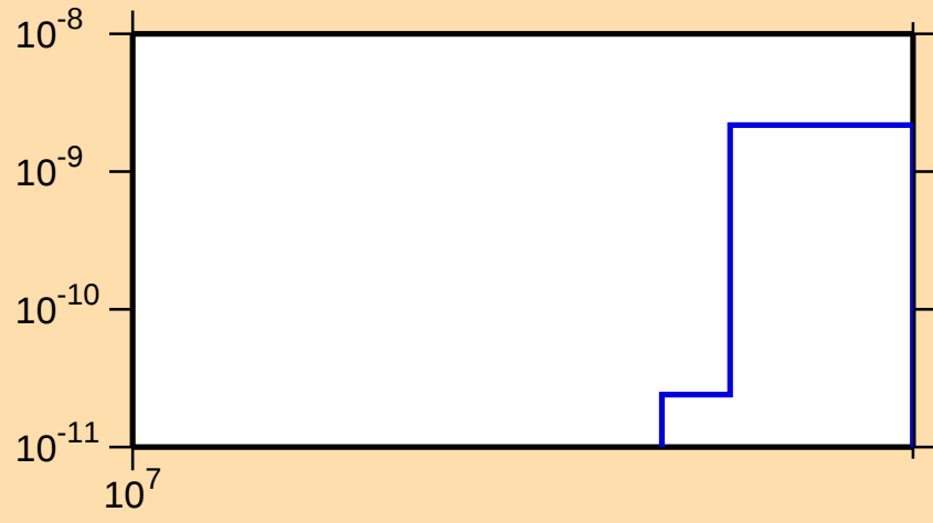
\sigma vs. E for ^{97}\text{Tc}(\text{mt } 45)
