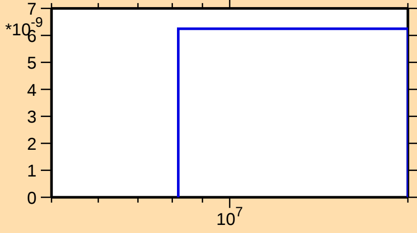
\sigma vs. E for ^{97}\text{Tc}(n,\text{nt})
