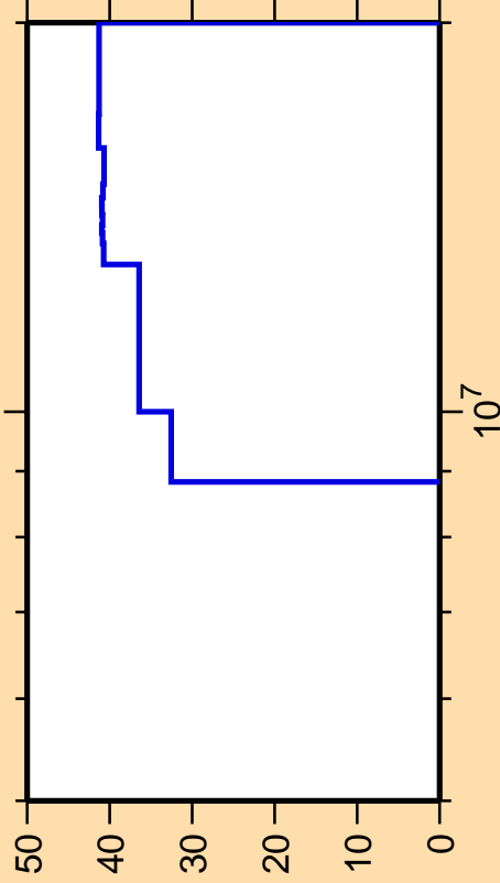
\Delta\sigma/\sigma vs. E for ^{99}\text{Tc}(n,\gamma)
