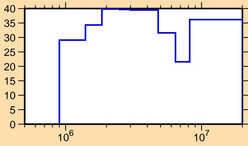
\Delta\sigma/\sigma vs. E for ^{99}\text{Tc}(n,\gamma)
