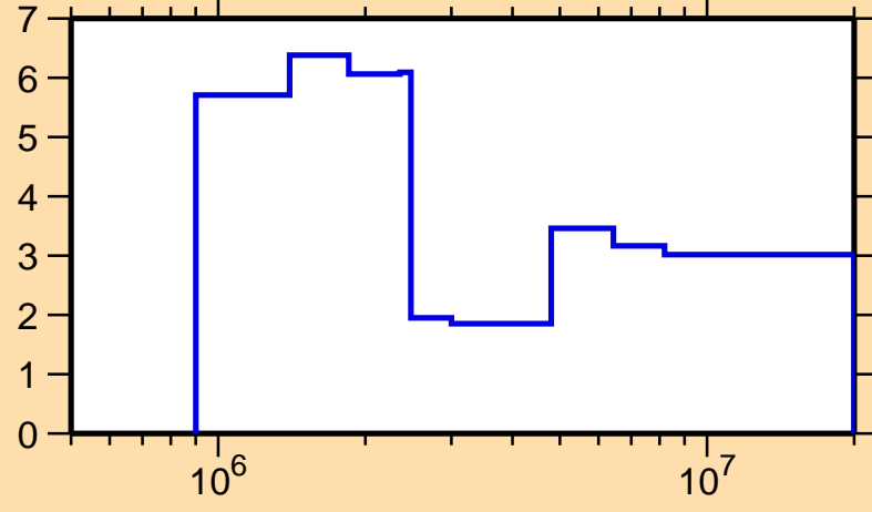
\Delta\sigma/\sigma vs. E for ^{99}\text{Tc}(n,el.)
