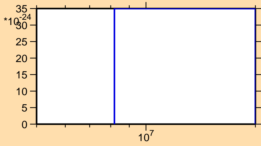
\sigma vs. E for ^{99}\text{Tc}(n,3n\alpha)
