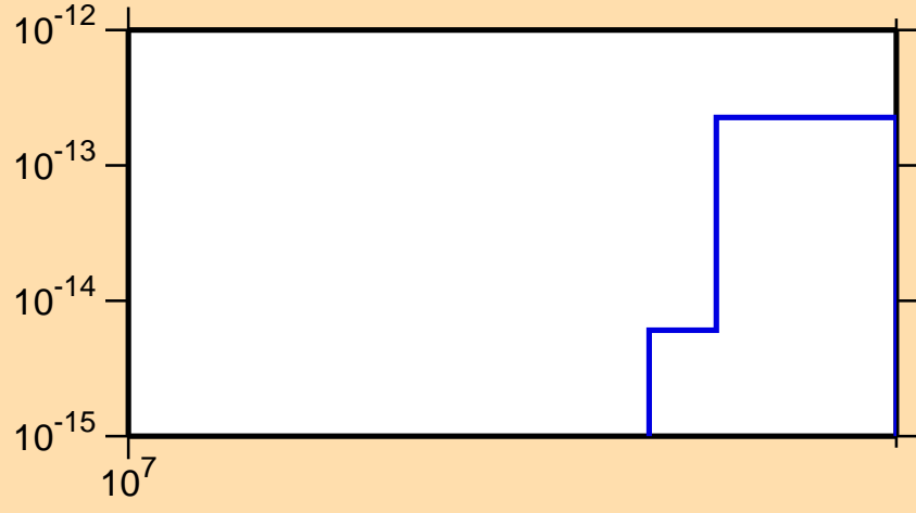
\sigma vs. E for ^{100}\text{Tc}(\text{mt117})
