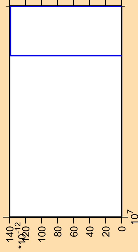
\Delta\sigma/\sigma vs. E for ^{100}\text{Tc}(\text{mt } 11)
