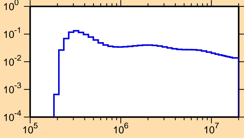
\sigma vs. E for ^{100}\text{Tc}(n,n_2)
