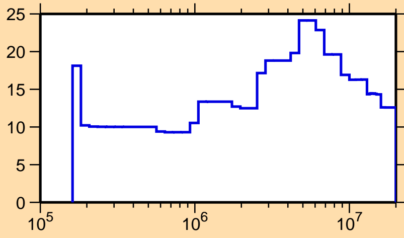
\Delta\sigma/\sigma vs. E for ^{100}\text{Tc}(n,n_1)
