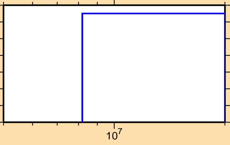
\sigma vs. E for ^{100}\text{Tc}(n,2np)
