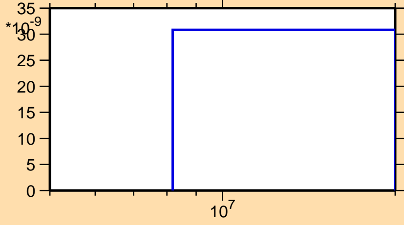
\sigma vs. E for ^{100}\text{Tc}(n,nt)
