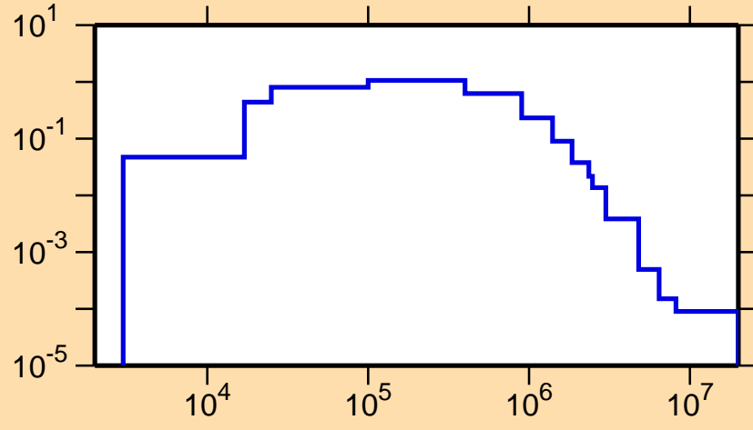
\sigma vs. E for ^{101}\text{Tc}(n,n_1)
