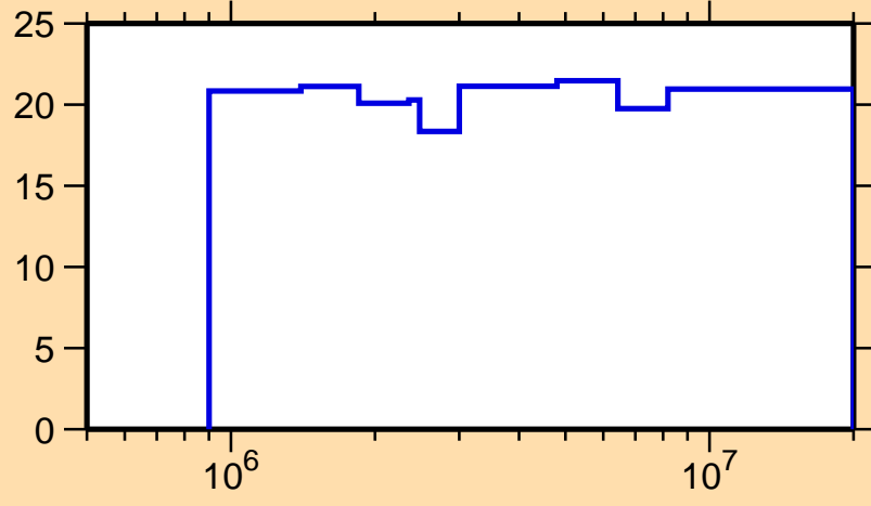
\Delta\sigma/\sigma vs. E for ^{102}\text{Tc}(n,\gamma)
