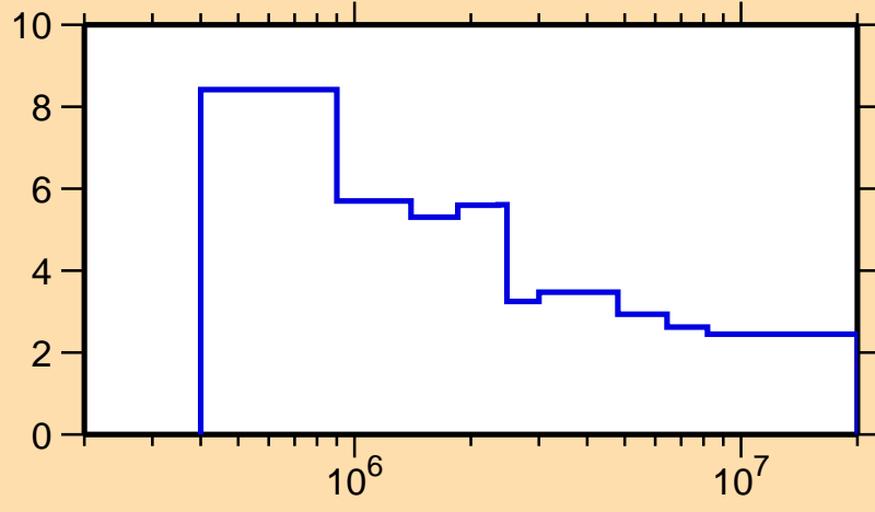
\Delta\sigma/\sigma vs. E for ^{102}\text{Tc}(n,n\text{onel.})
