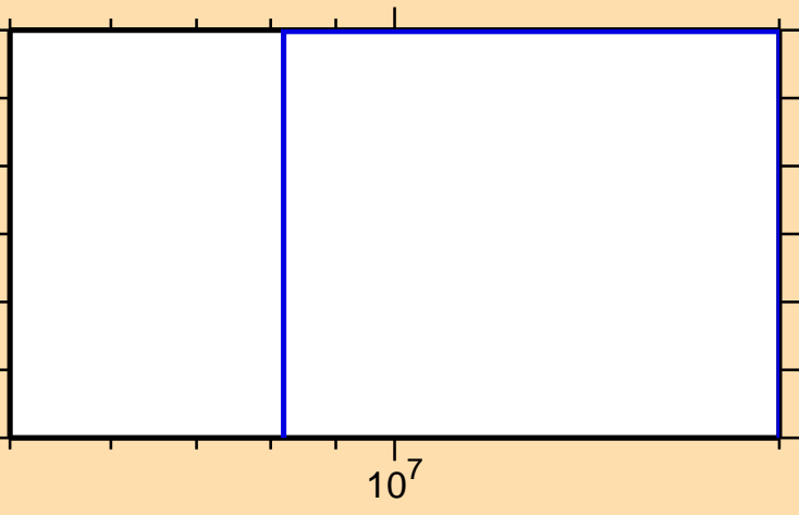
\sigma vs. E for ^{102}\text{Tc}(n,2n\alpha)
