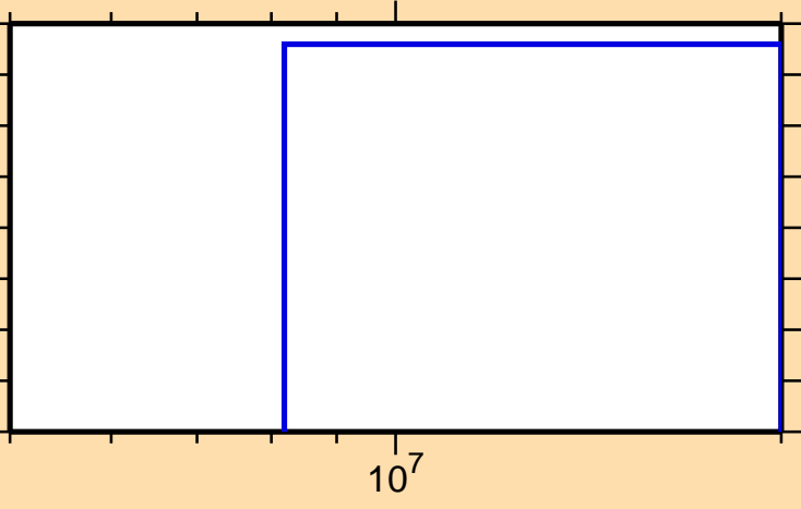
\sigma vs. E for ^{102}\text{Tc}(n,3n)
