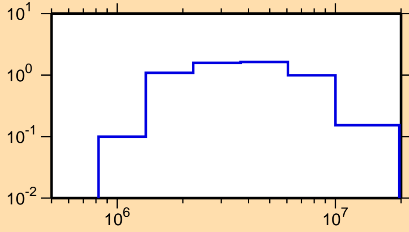
\sigma vs. E for ^{104}\text{Tc}(n,n\text{cont.})
