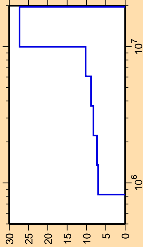
\Delta\sigma/\sigma vs. E for ^{104}\text{Tc}(n,n\text{cont.})
