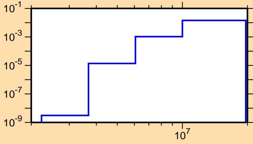
\sigma vs. E for ^{104}\text{Tc}(n,p)
