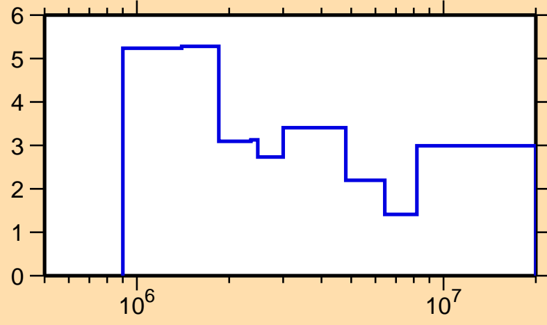
\Delta\sigma/\sigma vs. E for ^{104}\text{Tc}(n,\text{tot.})
