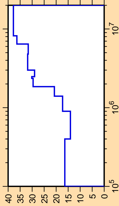
\Delta\sigma/\sigma vs. E for ^{104}\text{Tc}(n,n_2)
