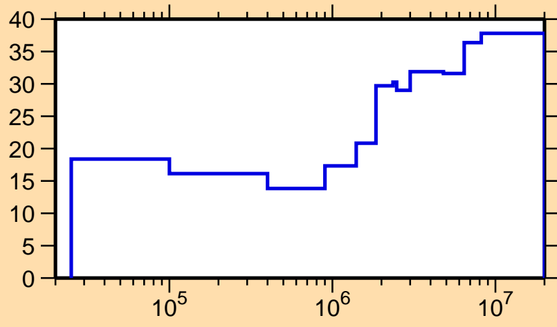
\Delta\sigma/\sigma vs. E for ^{104}\text{Tc}(n,n_1)
