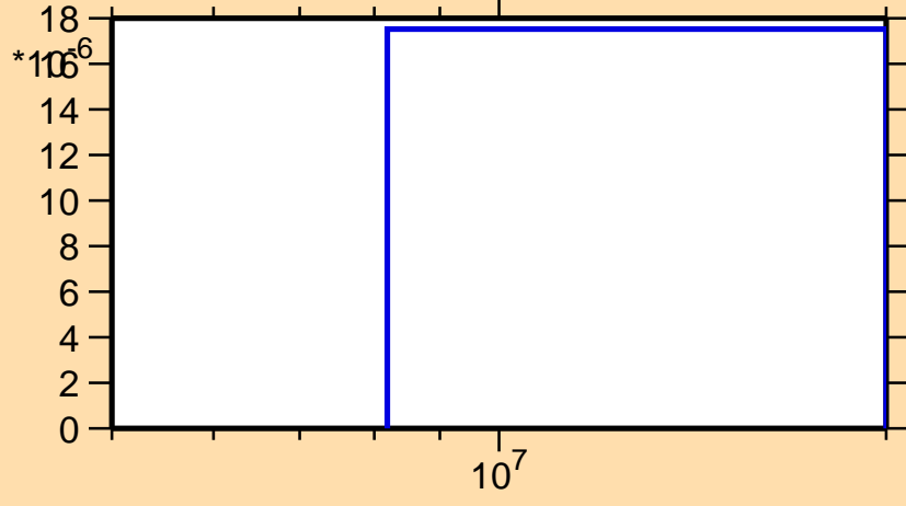
\sigma vs. E for ^{104}\text{Tc}(n,n\alpha)
