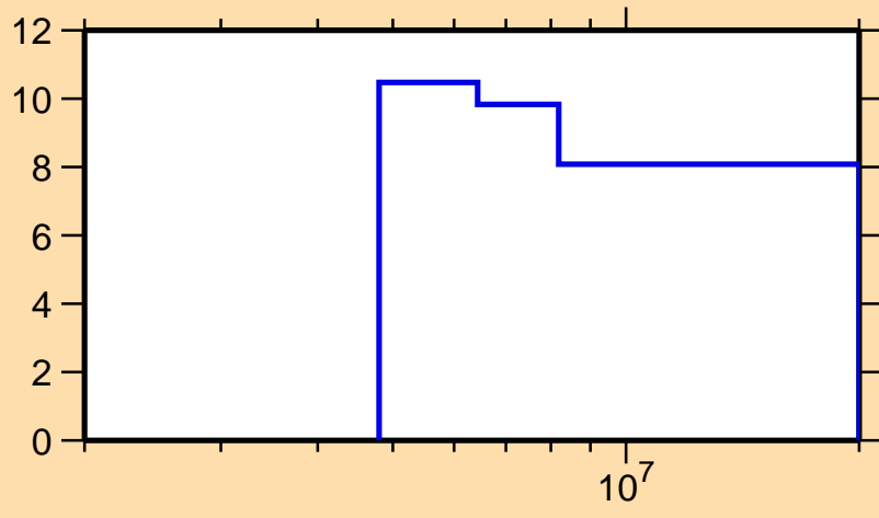
\Delta\sigma/\sigma vs. E for ^{104}\text{Tc}(n,2n)
