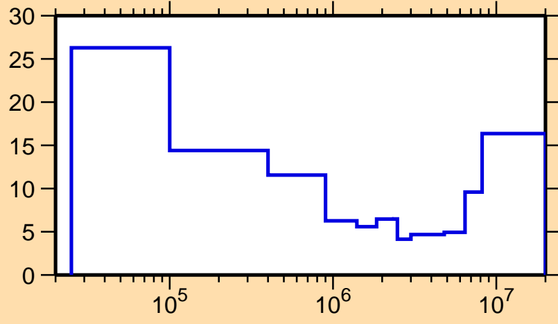
\Delta\sigma/\sigma vs. E for ^{104}\text{Tc}(n,\text{inel.})
