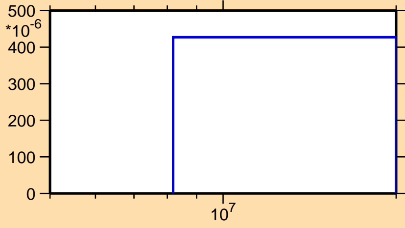
\sigma vs. E for ^{104}\text{Tc}(n,np)
