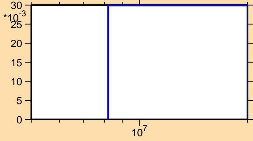
\sigma vs. E for ^{104}\text{Tc}(n,3n)
