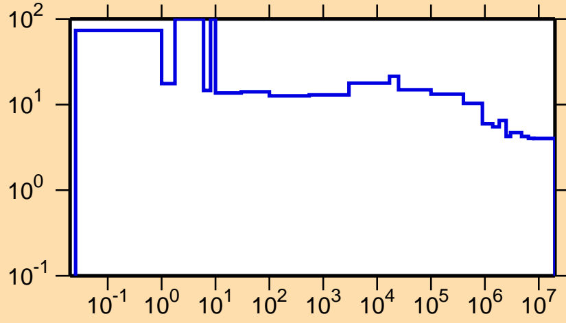
\Delta\sigma/\sigma vs. E for ^{104}\text{Tc}(n,\text{nonel.})
