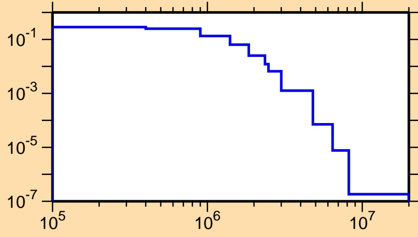
\sigma vs. E for ^{104}\text{Tc}(n,n_2)
