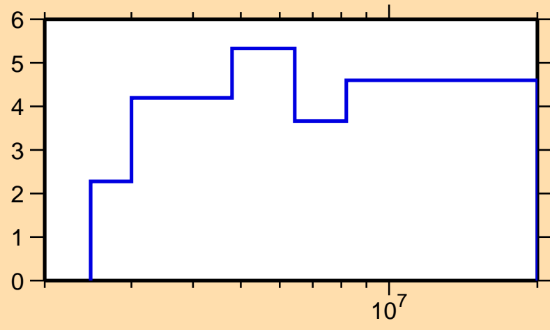
\Delta\sigma/\sigma vs. E for ^{104}\text{Tc}(n,\text{el.})
