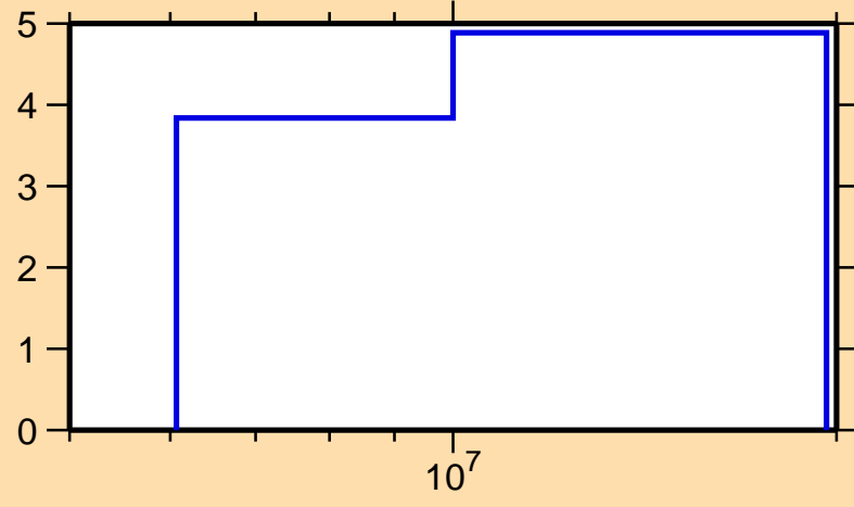
\Delta\sigma/\sigma vs. E for ^{107}\text{Tc}(n,\text{tot.})
