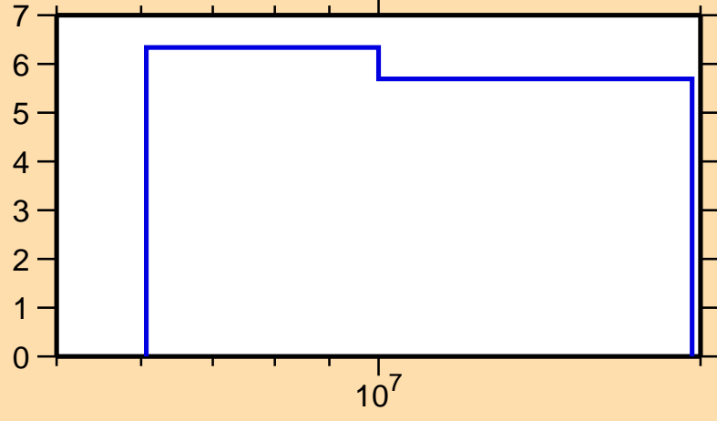
\Delta\sigma/\sigma vs. E for ^{107}\text{Tc}(n,\text{el.})
