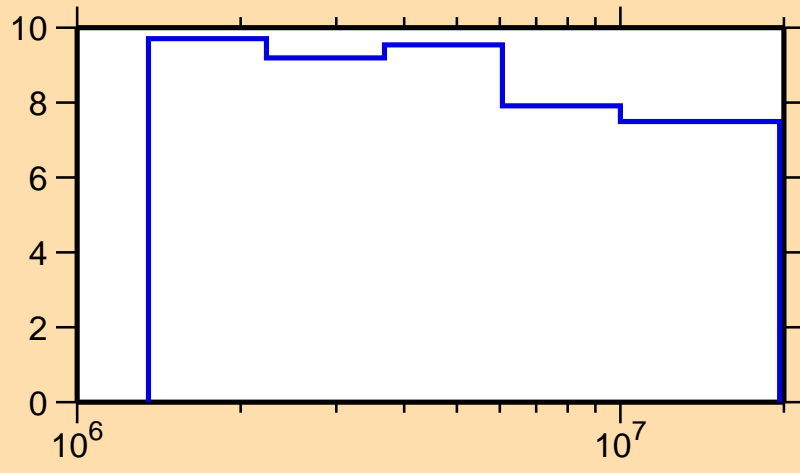
\Delta\sigma/\sigma vs. E for ^{107}\text{Tc}(n, n_{\text{nonel}})
