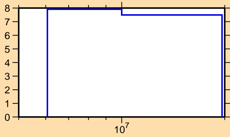
\Delta\sigma/\sigma vs. E for ^{107}\text{Tc}(n,\text{nonel.})
