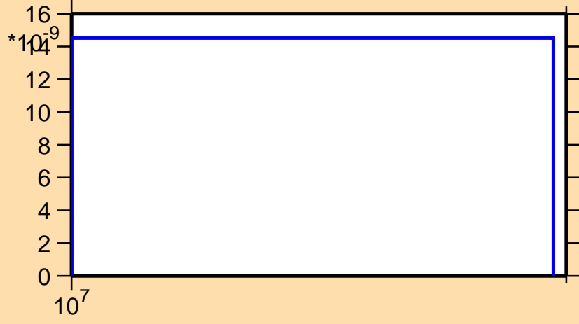
\sigma vs. E for ^{107}\text{Tc}(n,nt)
