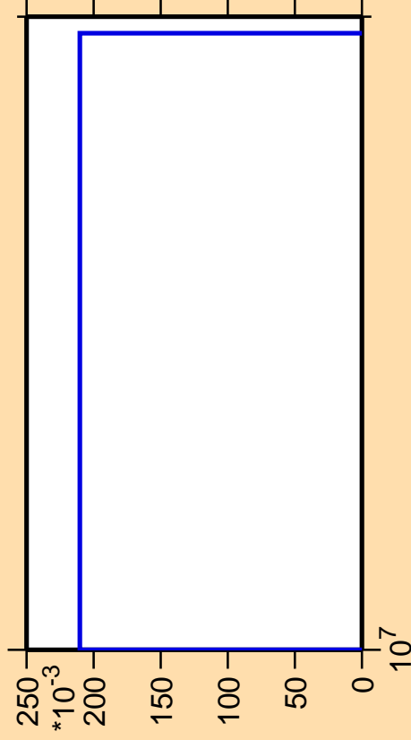
\Delta\sigma/\sigma vs. E for ^{107}\text{Tc}(n,2n\alpha)
