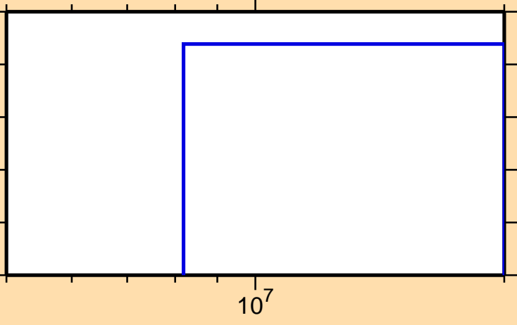
\sigma vs. E for ^{107}\text{Tc}(n,2n\alpha)
