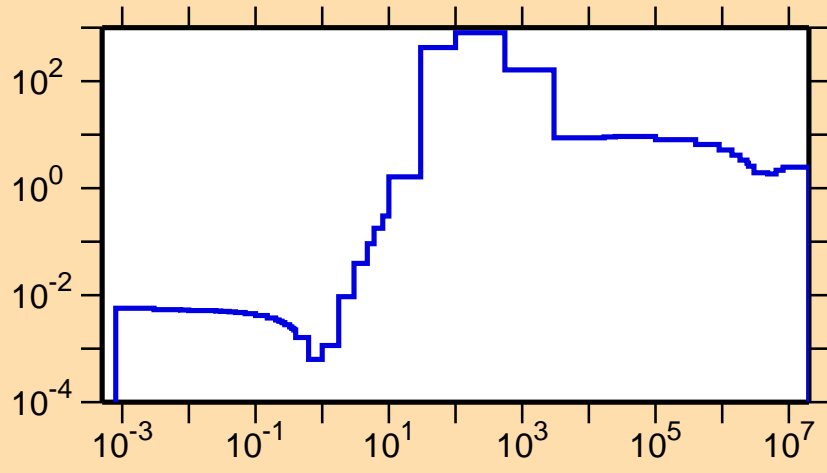
\sigma vs. E for ^{107}\text{Tc}(n,\text{el.})
