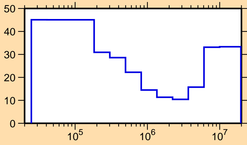
\Delta\sigma/\sigma vs. E for ^{108}\text{Tc}(n,\text{inel.})
