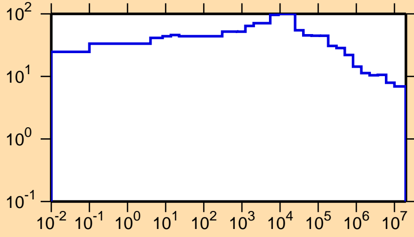
\Delta\sigma/\sigma vs. E for ^{108}\text{Tc}(n,\text{nonel.})
