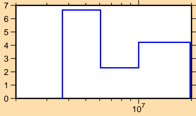
\Delta\sigma/\sigma vs. E for ^{108}\text{Tc}(n,\text{tot.})
