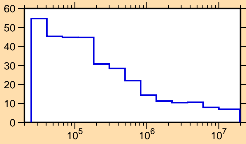
\Delta\sigma/\sigma vs. E for ^{108}\text{Tc}(n,\text{nonel.})
