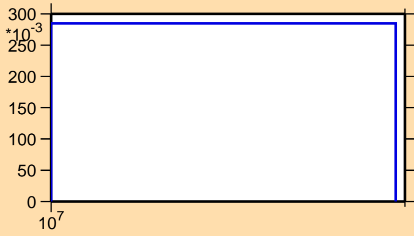
\sigma vs. E for ^{108}\text{Tc}(n,3n)
