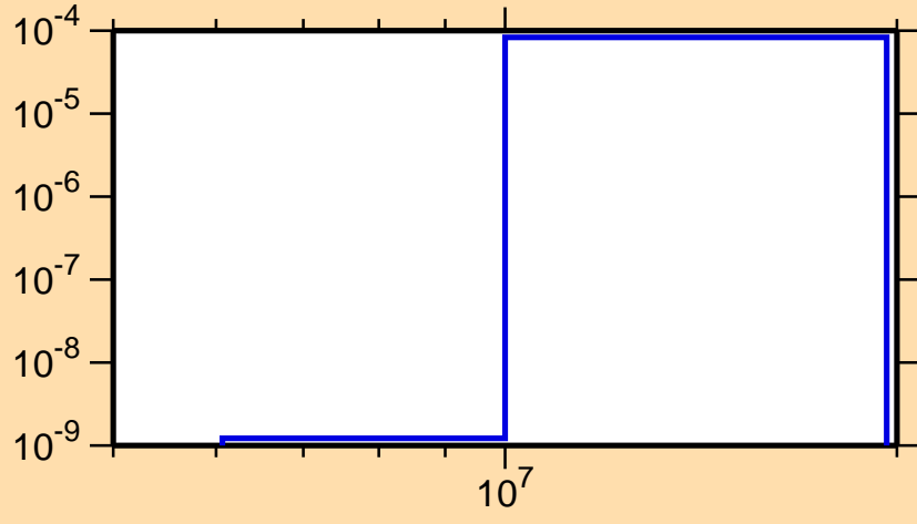
\sigma vs. E for ^{108}\text{Tc}(n,\alpha)
