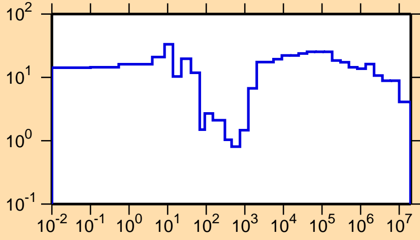
\Delta\sigma/\sigma vs. E for ^{108}\text{Tc}(n,\text{el.})
