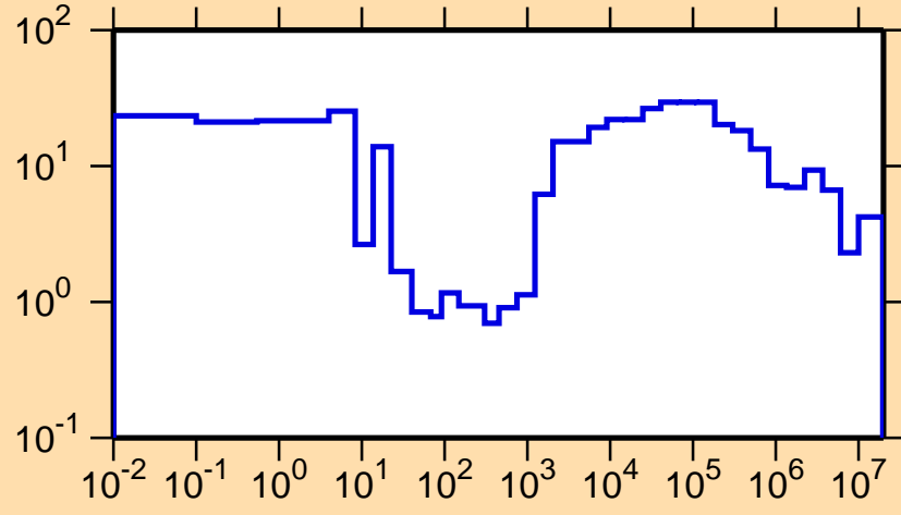
\Delta\sigma/\sigma vs. E for ^{108}\text{Tc}(n,\text{tot.})
