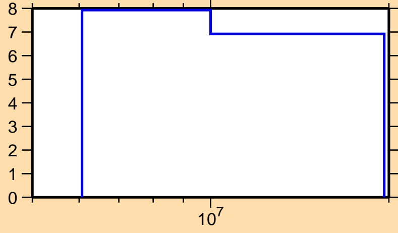
\Delta\sigma/\sigma vs. E for ^{108}\text{Tc}(n,\text{nonel.})
