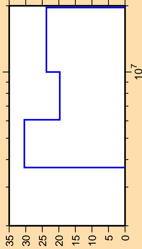
\Delta\sigma/\sigma vs. E for ^{108}\text{Tc}(n,2n)
