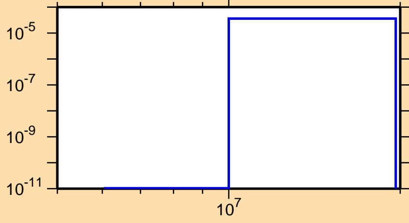
\sigma vs. E for ^{108}\text{Tc}(n,t)
