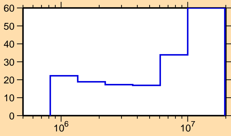
\Delta\sigma/\sigma vs. E for ^{108}\text{Tc}(n,n\text{cont.})
