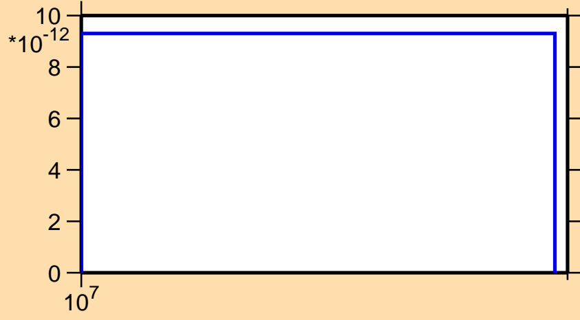
\sigma vs. E for ^{108}\text{Tc}(n,2n\alpha)
