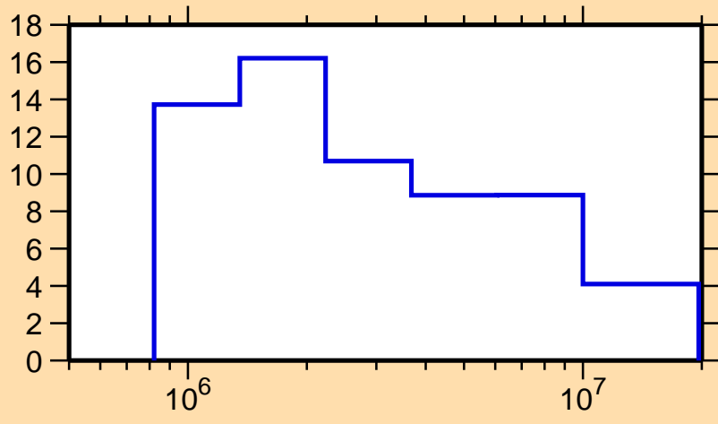
\Delta\sigma/\sigma vs. E for ^{108}\text{Tc}(n,\text{el.})
