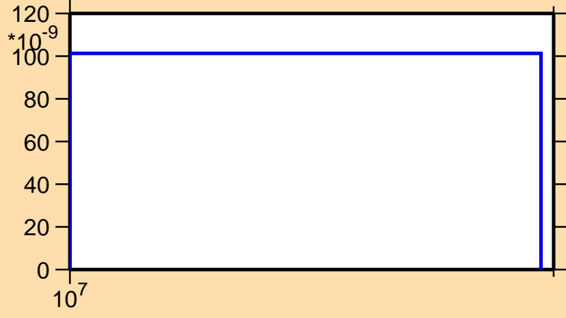
\sigma vs. E for ^{108}\text{Tc}(n,\text{nd})
