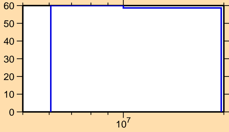
\Delta\sigma/\sigma vs. E for ^{108}\text{Tc}(n,p)
