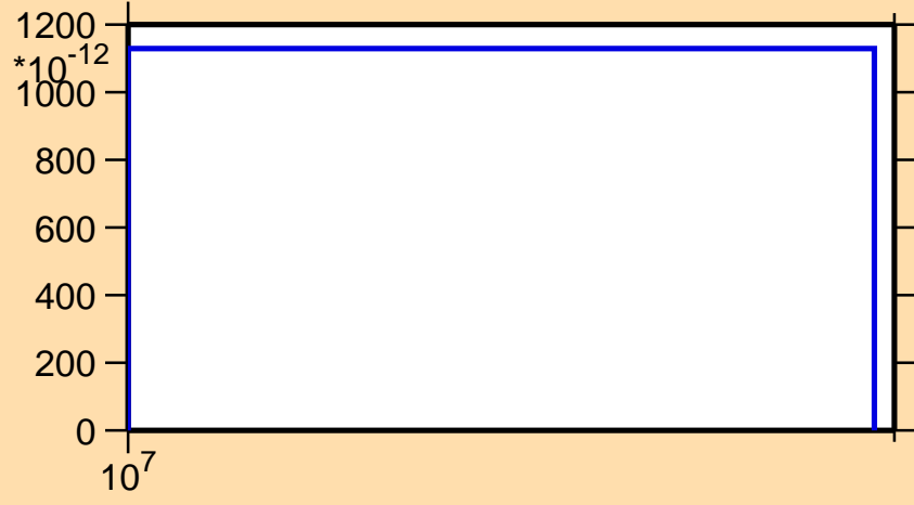
\sigma vs. E for ^{108}\text{Tc}(n,2np)
