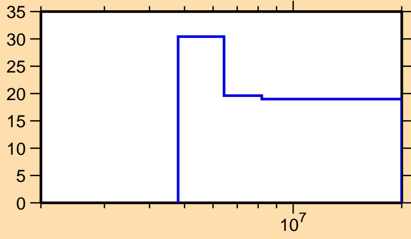
\Delta\sigma/\sigma vs. E for ^{108}\text{Tc}(n,2n)
