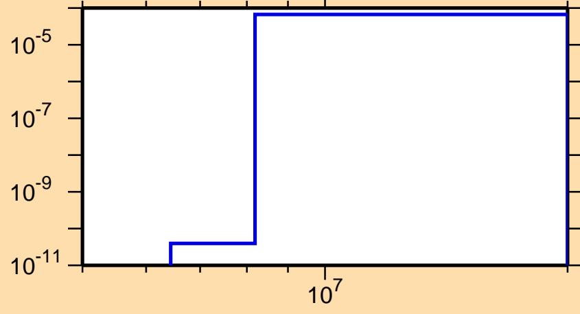
\sigma vs. E for ^{108}\text{Tc}(n,\alpha)
