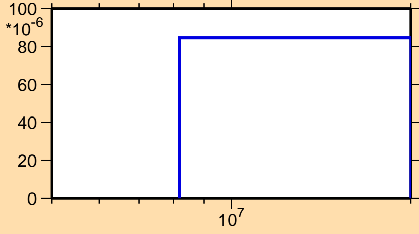
\sigma vs. E for ^{108}\text{Tc}(n,d)
