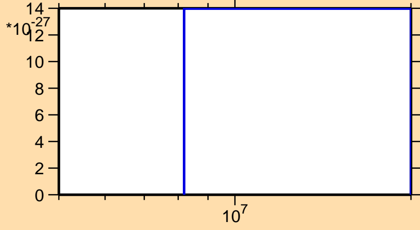
\sigma vs. E for ^{108}\text{Tc}(\text{mt } 11)
