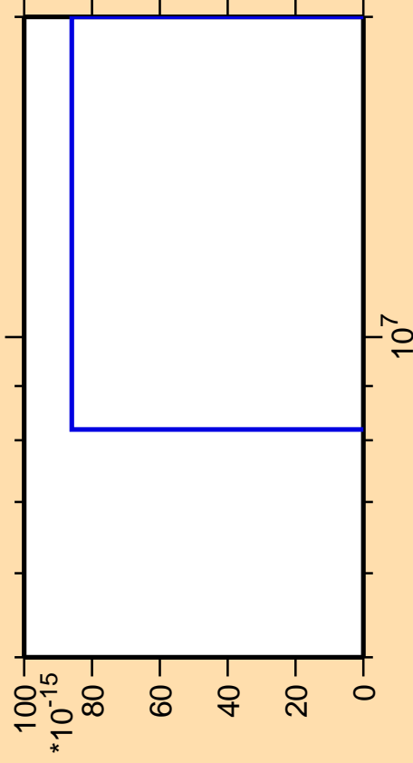
\Delta\sigma/\sigma vs. E for ^{108}\text{Tc}(\text{mt } 11)
