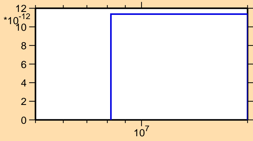
\sigma vs. E for ^{108}\text{Tc}(n,2n\alpha)
