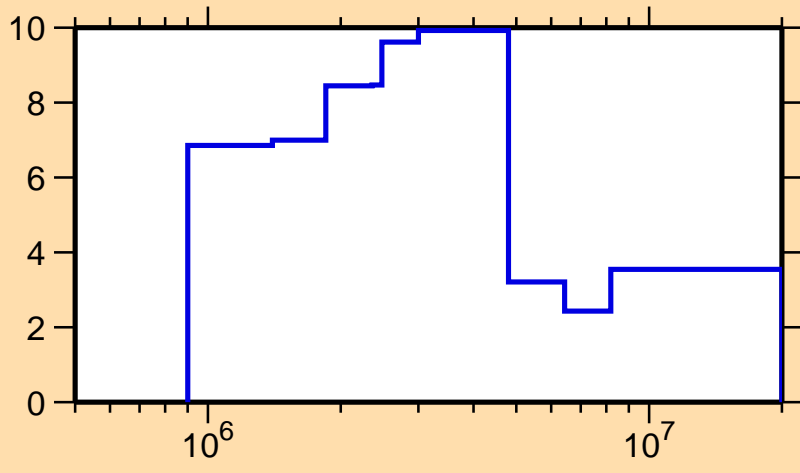
\Delta\sigma/\sigma vs. E for ^{108}\text{Tc}(n,\text{tot.})
