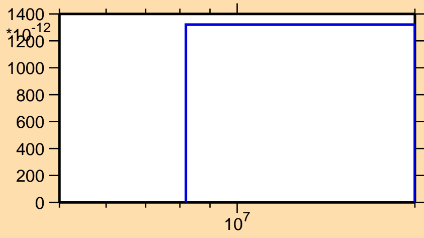
\sigma vs. E for ^{108}\text{Tc}(n,2np)
