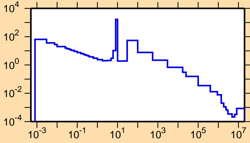
\sigma vs. E for ^{108}\text{Tc}(n,\gamma)
