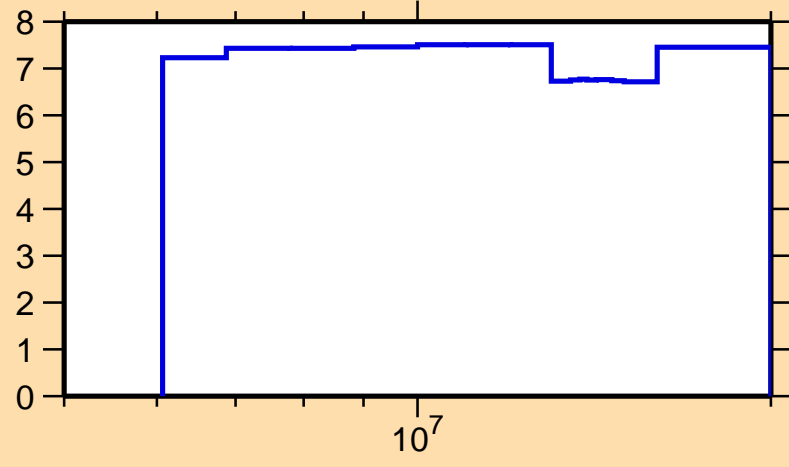
\Delta\sigma/\sigma vs. E for ^{109}\text{Tc}(n,\text{nonel.})
