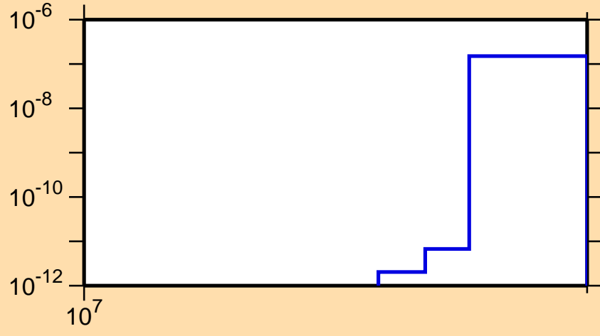
\sigma vs. E for ^{109}\text{Tc}(n,\text{nd})
