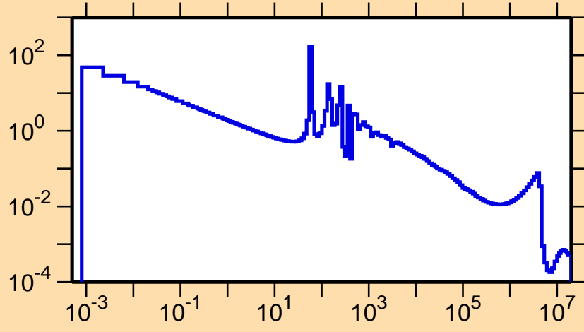
\sigma vs. E for ^{109}\text{Tc}(n,\gamma)
