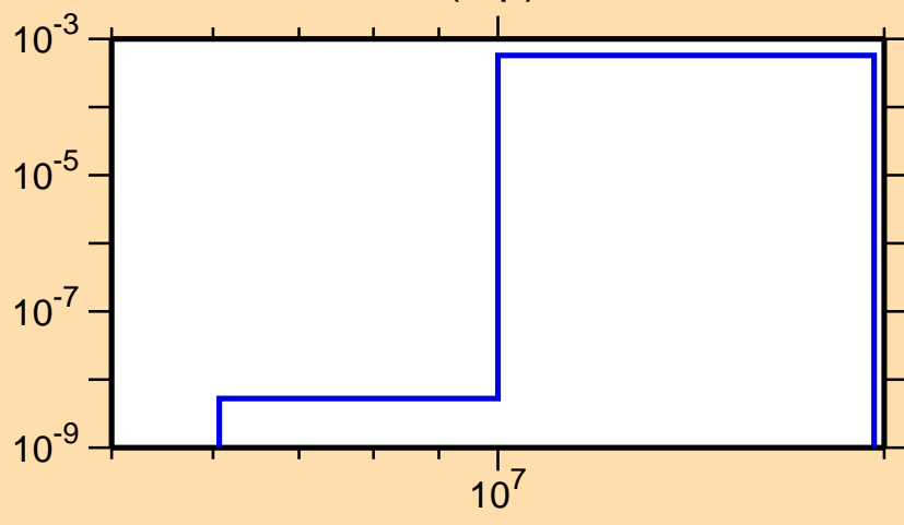
\sigma vs. E for ^{109}\text{Tc}(n,p)
