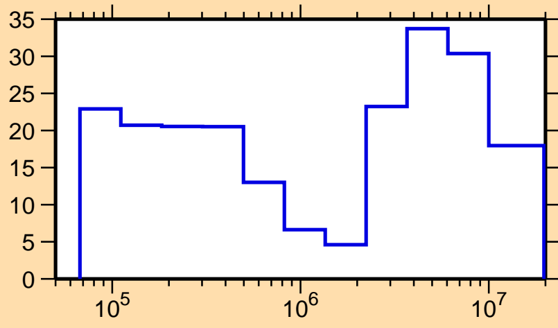
\Delta\sigma/\sigma vs. E for ^{109}\text{Tc}(n,n_1)
