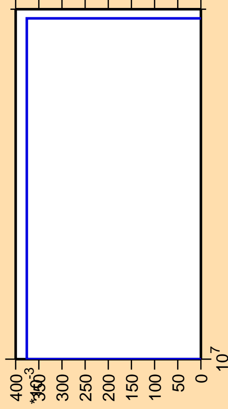
\Delta\sigma/\sigma vs. E for ^{109}\text{Tc}(n,2np)
