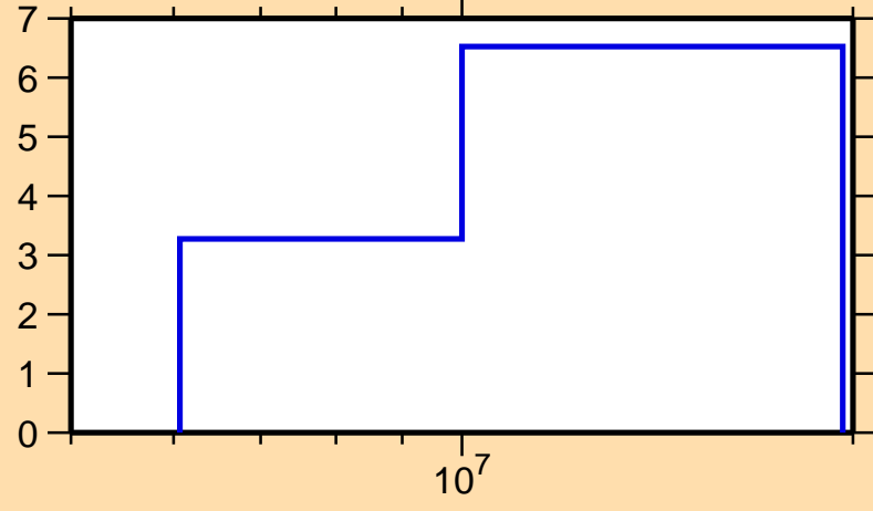
\Delta\sigma/\sigma vs. E for ^{109}\text{Tc}(n,el.)
