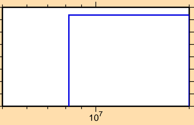
\sigma vs. E for ^{109}\text{Tc}(n,2n\alpha)
