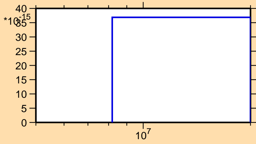
\sigma vs. E for ^{109}\text{Tc}(n,2n\alpha)
