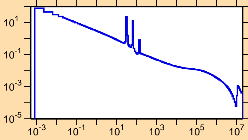
\sigma vs. E for ^{108}\text{Te}(n,\gamma)
