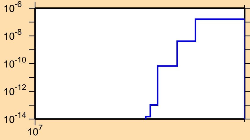
\sigma vs. E for ^{108}\text{Te}(n,\text{nd})
