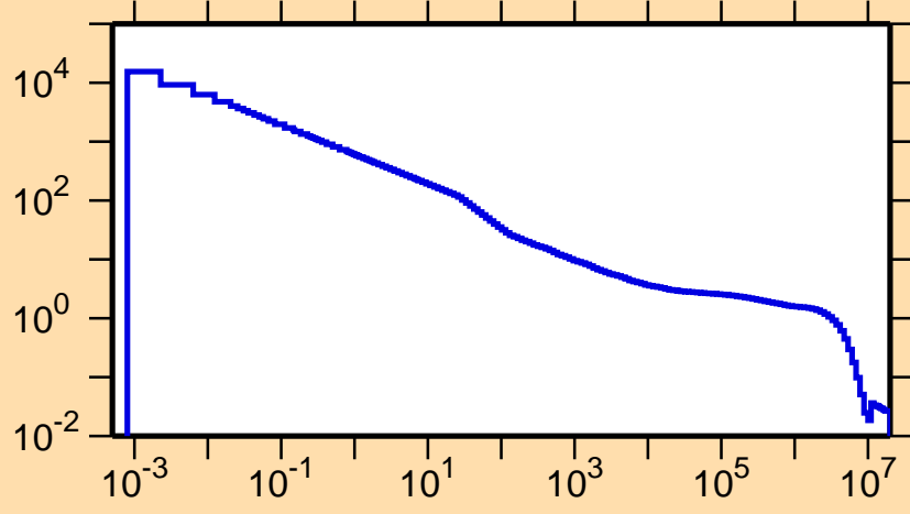
\sigma vs. E for ^{108}\text{Te}(n,p)
