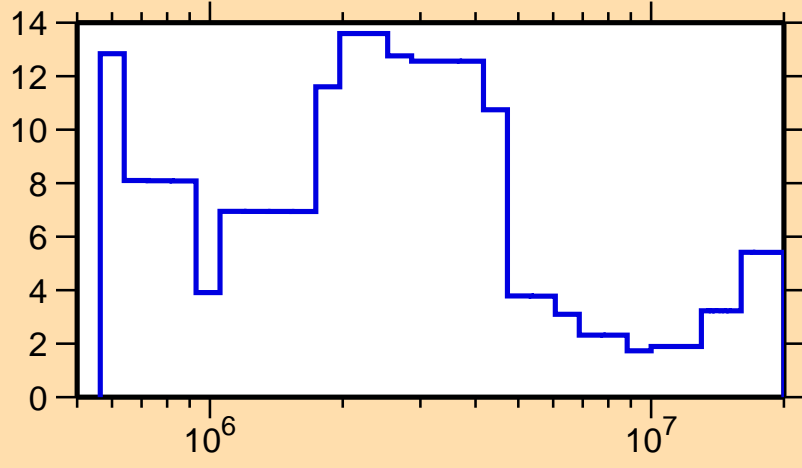
\Delta\sigma/\sigma vs. E for ^{108}\text{Te}(n,\text{tot.})
