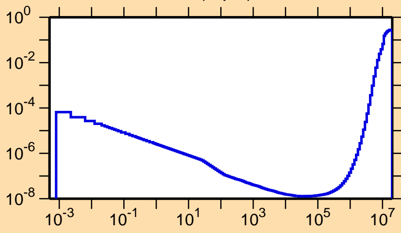
\sigma vs. E for ^{108}\text{Te}(n,p\alpha)
