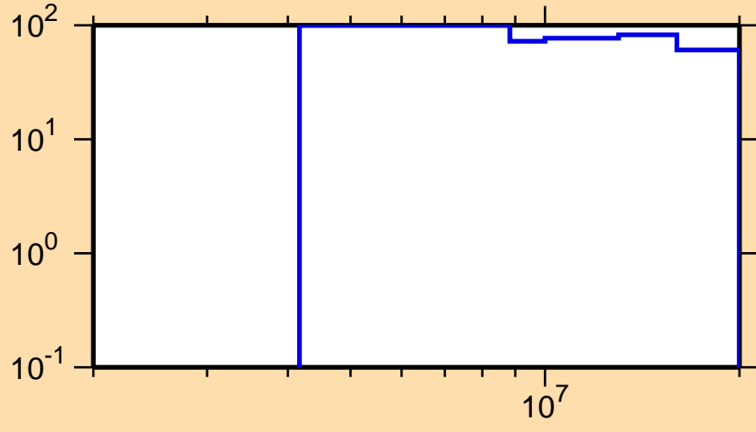
\Delta\sigma/\sigma vs. E for ^{108}\text{Te}(n,n\text{cont.})
