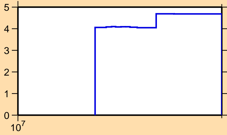
\Delta\sigma/\sigma vs. E for ^{108}\text{Te}(n,\text{el.})
