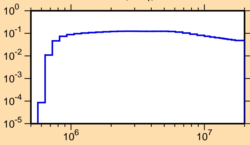
\sigma vs. E for ^{108}\text{Te}(n,n_1)
