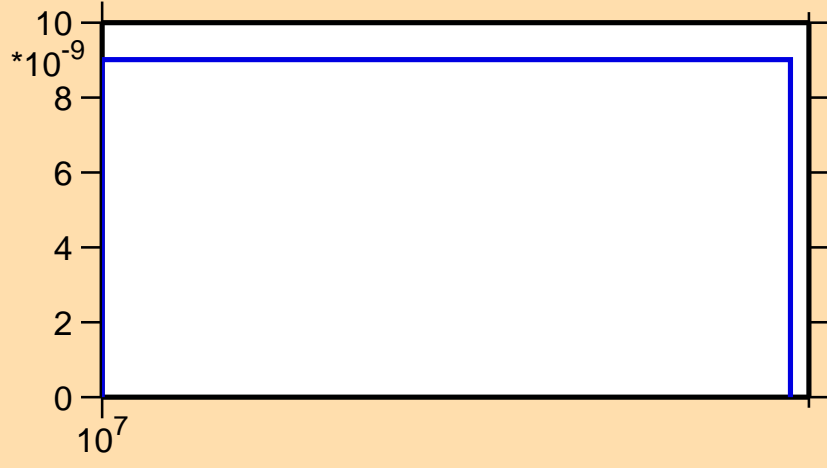
\sigma vs. E for ^{108}\text{Te} (mt 34)
