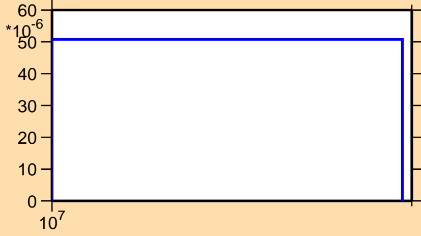
\sigma vs. E for ^{108}\text{Te}(n,2n)
