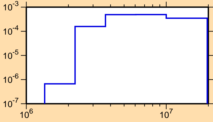
\sigma vs. E for ^{108}\text{Te}(n,n_3)
