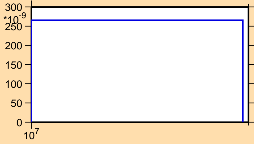
\sigma vs. E for ^{108}\text{Te}(n,2n\alpha)
