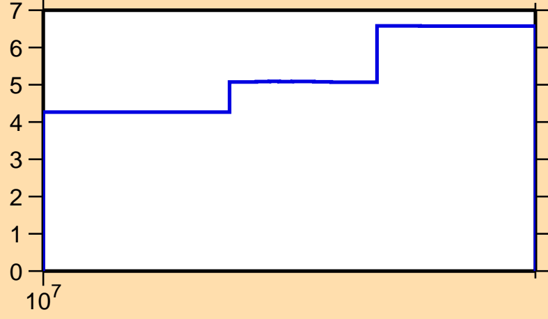
\Delta\sigma/\sigma vs. E for ^{109}\text{Te}(n,\text{tot.})
