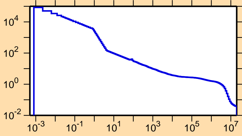
\sigma vs. E for ^{109}\text{Te}(n,p)
