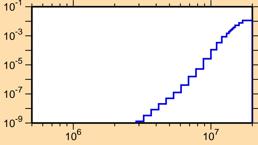
\sigma vs. E for ^{109}\text{Te}(n,\text{He}3)
