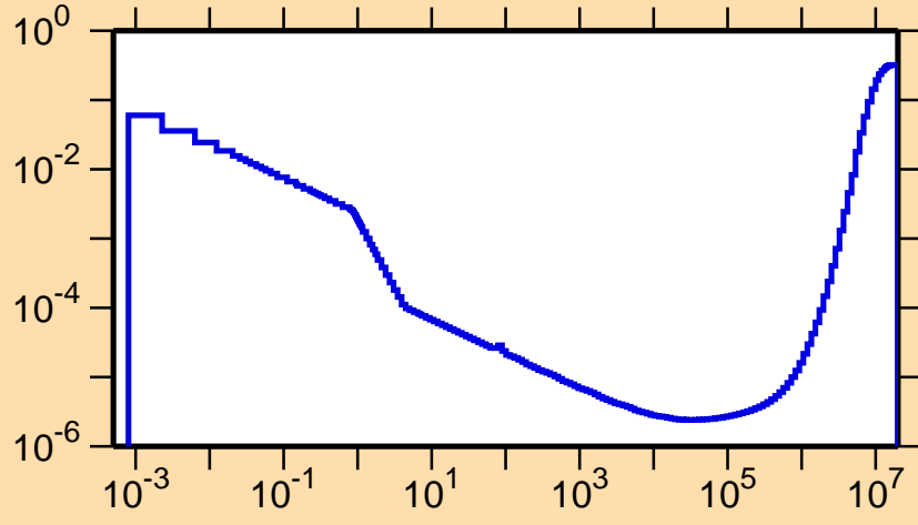
\sigma vs. E for ^{109}\text{Te}(n,p\alpha)
