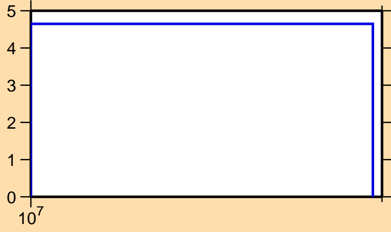
\Delta\sigma/\sigma vs. E for ^{109}\text{Te}(n,\text{el.})
