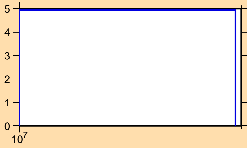
\Delta\sigma/\sigma vs. E for ^{109}\text{Te}(n,\text{tot.})
