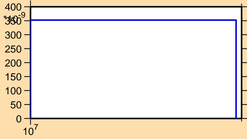
\sigma vs. E for ^{109}\text{Te}(n,2n\alpha)
