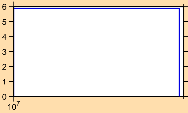
\Delta\sigma/\sigma vs. E for ^{109}\text{Te}(n,\text{nonel.})
