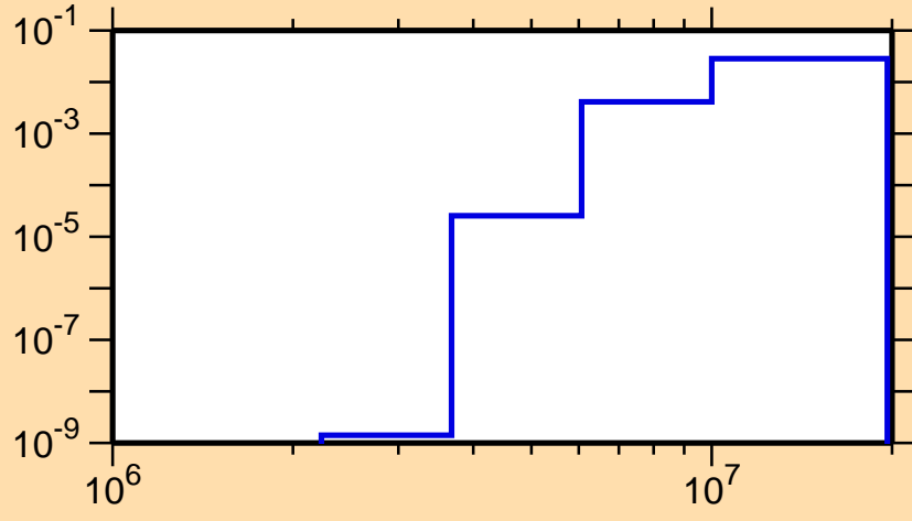
\sigma vs. E for ^{109}\text{Te}(n,n\alpha)
