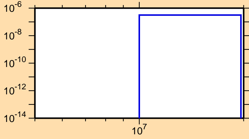
\sigma vs. E for ^{109}\text{Te}(\text{mt } 34)
