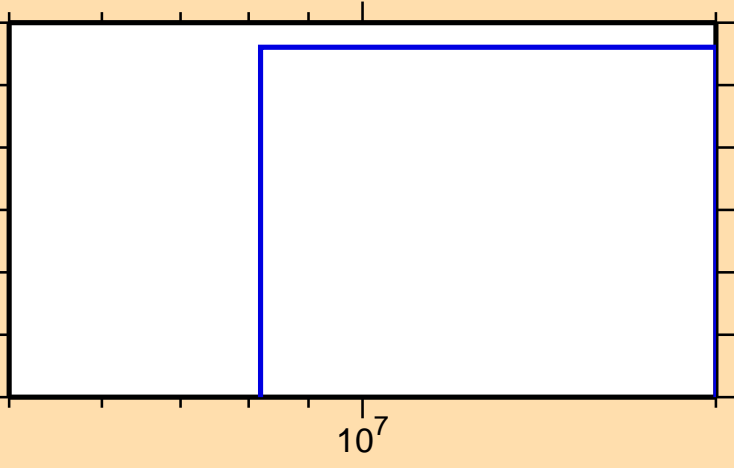
\sigma vs. E for ^{109}\text{Te}(n,nt)
