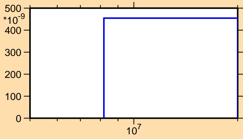
\sigma vs. E for ^{109}\text{Te}(\text{mt117})
