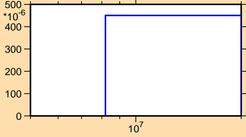
\sigma vs. E for ^{109}\text{Te}(n,2n)
