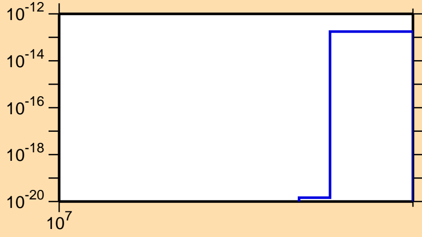
\sigma vs. E for ^{111}\text{Te}(n,nt)
