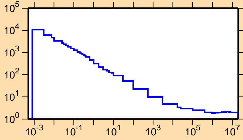
\sigma vs. E for ^{111}\text{Te}(n,\text{nonel.})
