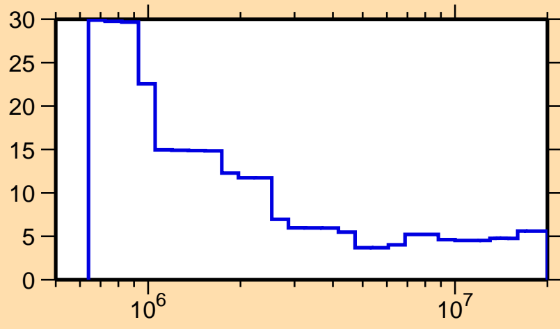
\Delta\sigma/\sigma vs. E for ^{112}\text{Te}(n,\text{nonel.})
