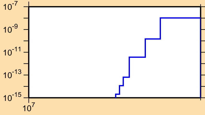
\sigma vs. E for ^{112}\text{Te} (mt 34)
