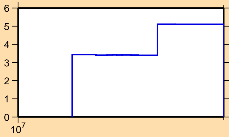
\Delta\sigma/\sigma vs. E for ^{112}\text{Te}(n,\text{tot.})
