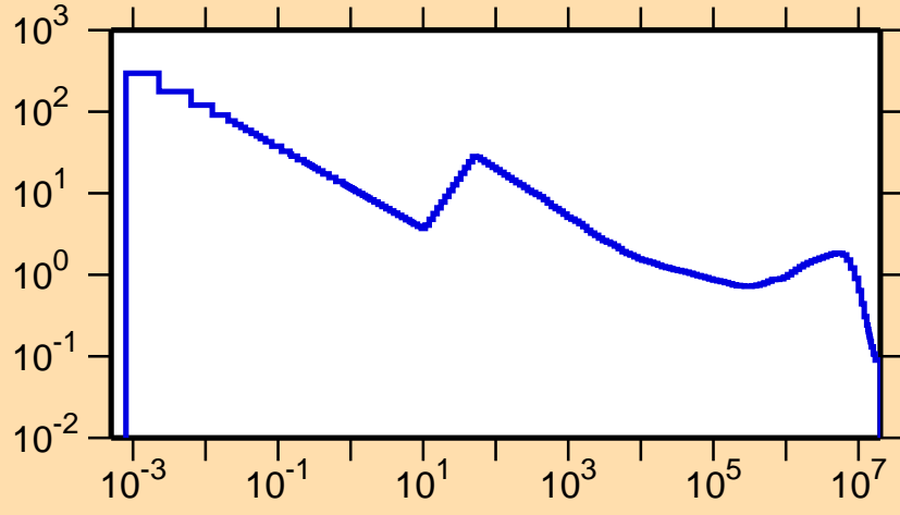
\sigma vs. E for ^{112}\text{Te}(n,p)
