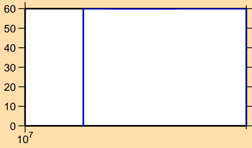
\Delta\sigma/\sigma vs. E for ^{112}\text{Te}(n,2n)
