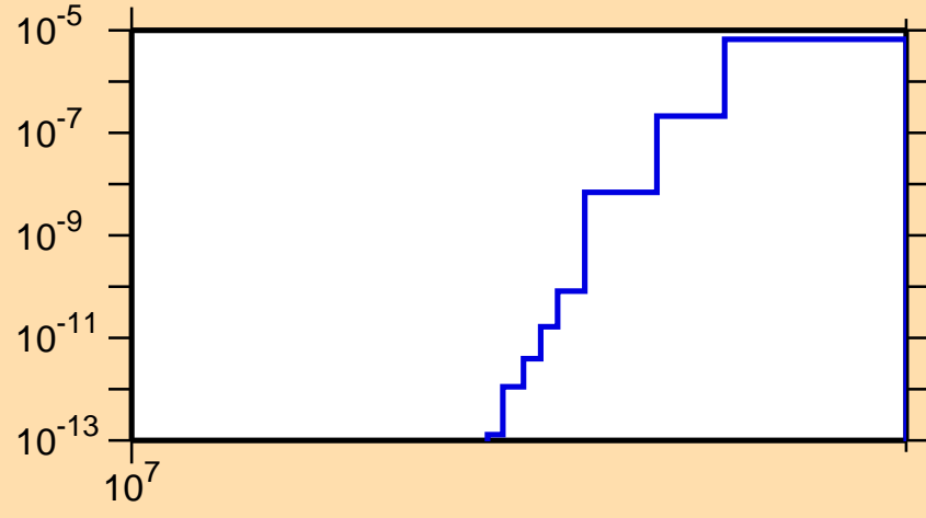
\sigma vs. E for ^{112}\text{Te}(n,\text{pt})
