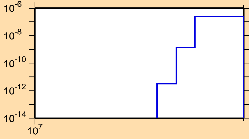
\sigma vs. E for ^{112}\text{Te}(n,\text{nd})
