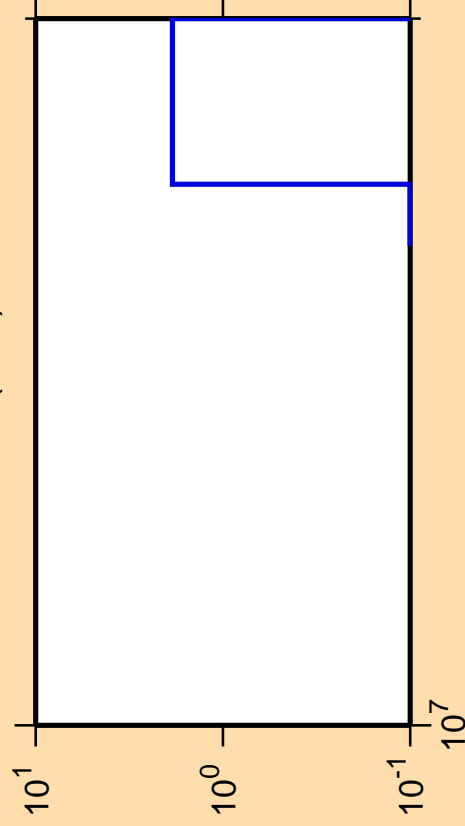
\Delta\sigma/\sigma vs. E for ^{112}\text{Te}(n,nt)
