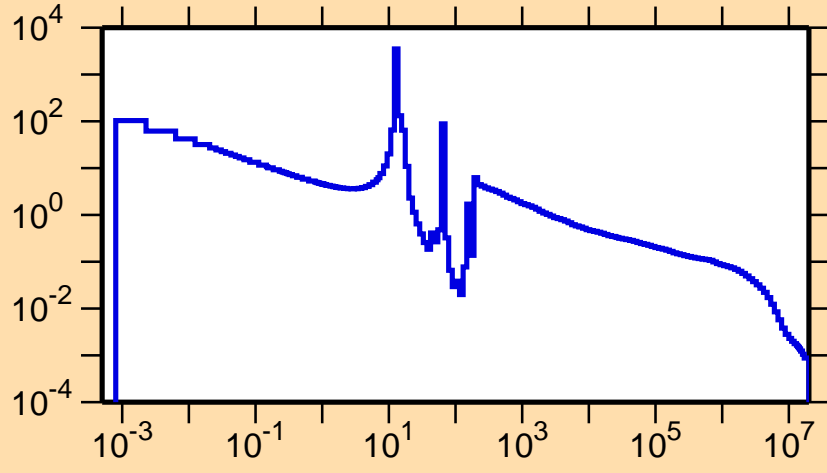
\sigma vs. E for ^{112}\text{Te}(n,\gamma)
