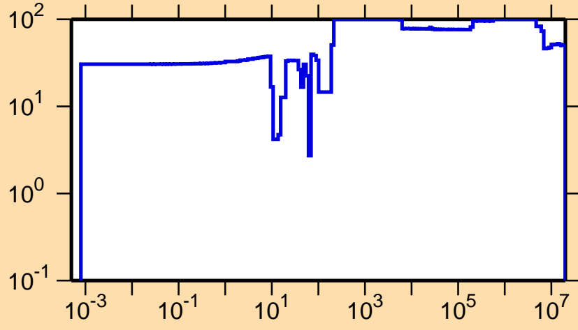
\Delta\sigma/\sigma vs. E for ^{112}\text{Te}(n,\gamma)
