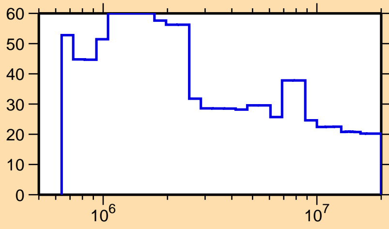
\Delta\sigma/\sigma vs. E for ^{112}\text{Te}(n,\text{inel.})
