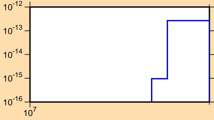
\sigma vs. E for ^{112}\text{Te}(n,nt)
