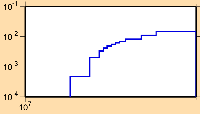
\sigma vs. E for ^{112}\text{Te}(n,2n)
