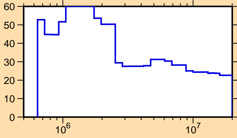
\Delta\sigma/\sigma vs. E for ^{112}\text{Te}(n,n_1)
