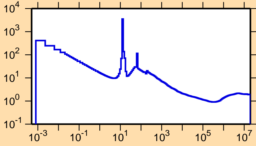
\sigma vs. E for ^{112}\text{Te}(n,\text{nonel.})
