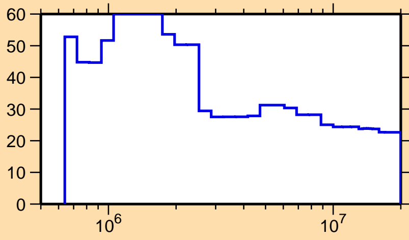
\Delta\sigma/\sigma vs. E for ^{112}\text{Te}(n,n_1)
