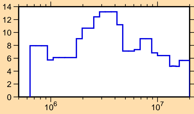
\Delta\sigma/\sigma vs. E for ^{112}\text{Te}(n,\text{el.})
