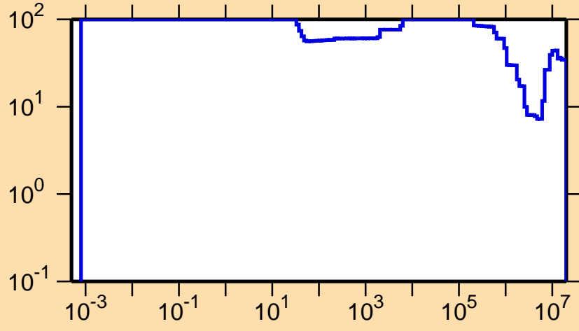
\Delta\sigma/\sigma vs. E for ^{112}\text{Te}(n,p)
