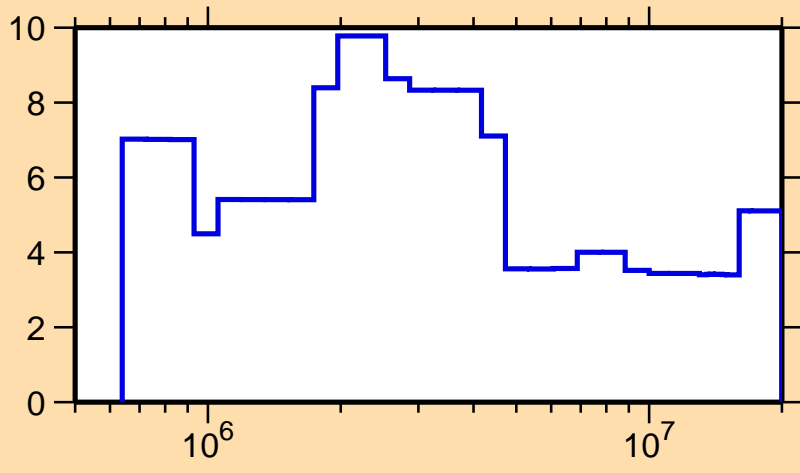
\Delta\sigma/\sigma vs. E for ^{112}\text{Te}(n,\text{tot.})
