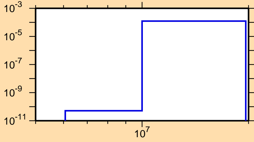
\sigma vs. E for ^{112}\text{Te}(n,pd)
