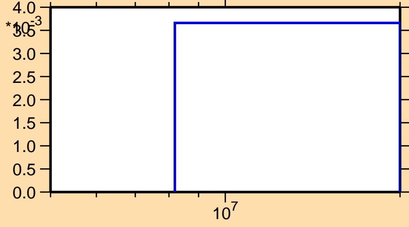
\sigma vs. E for ^{112}\text{Te}(n,2n)
